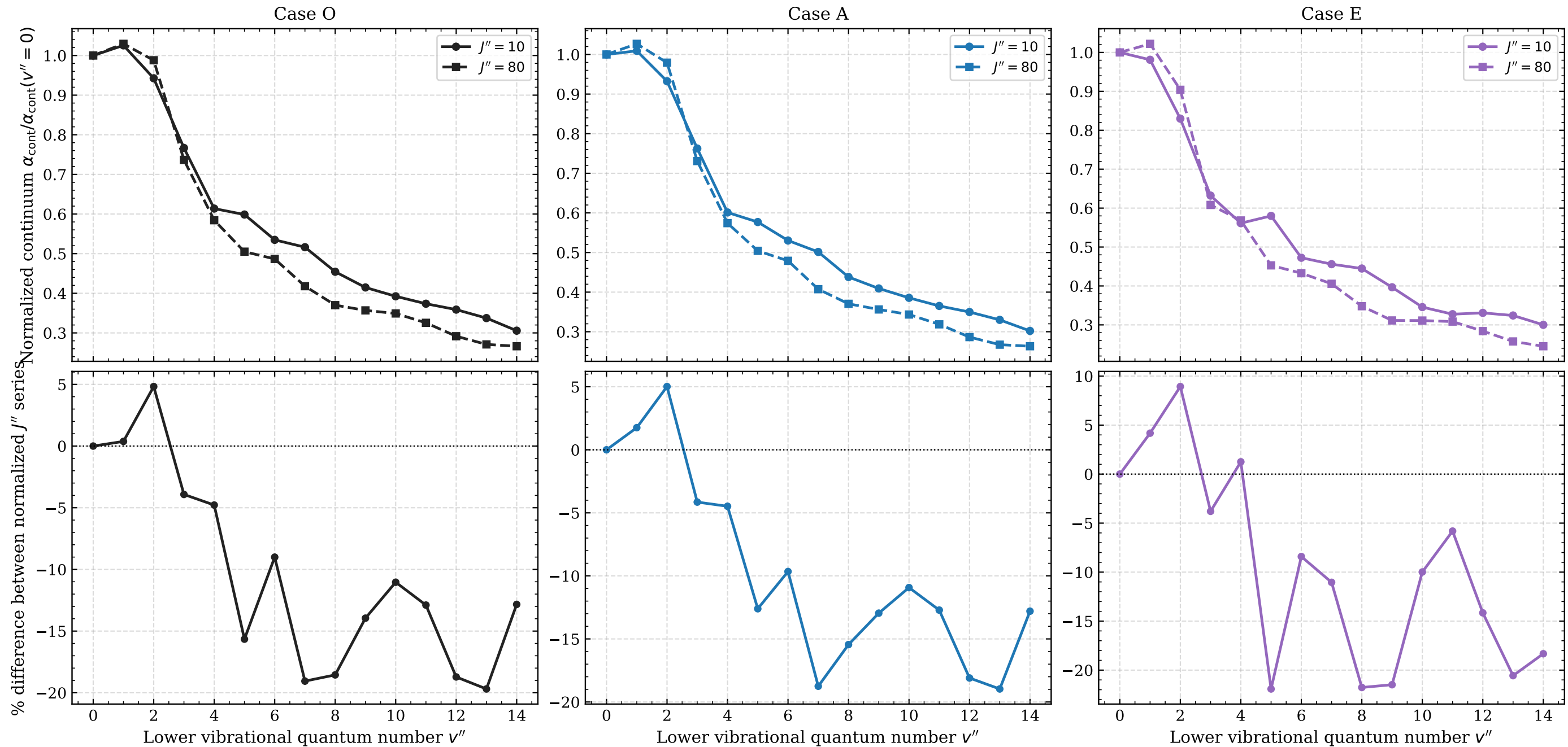
Continuum polarizability at 632.8 nm: Cases O, A, E (normalized; top = two J'' series, bottom = % difference)
