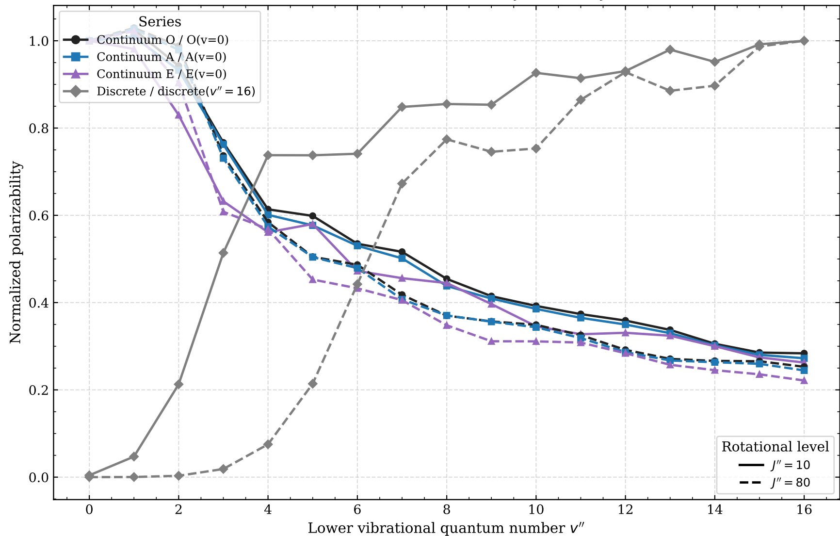
Continuum vs discrete at 632.8 nm: J'' = 10 and J'' = 80
