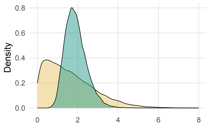
Weak shrinkage: Half-normal(6)
