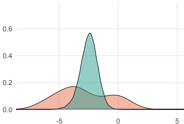
Weak shrinkage: Half-normal(6)
