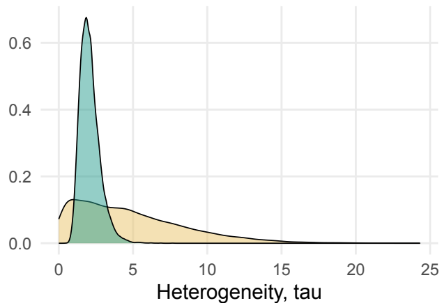
Weak shrinkage: Half-normal(6)
