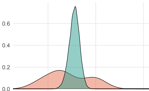
Strong shrinkage: Half-normal(0.67)
