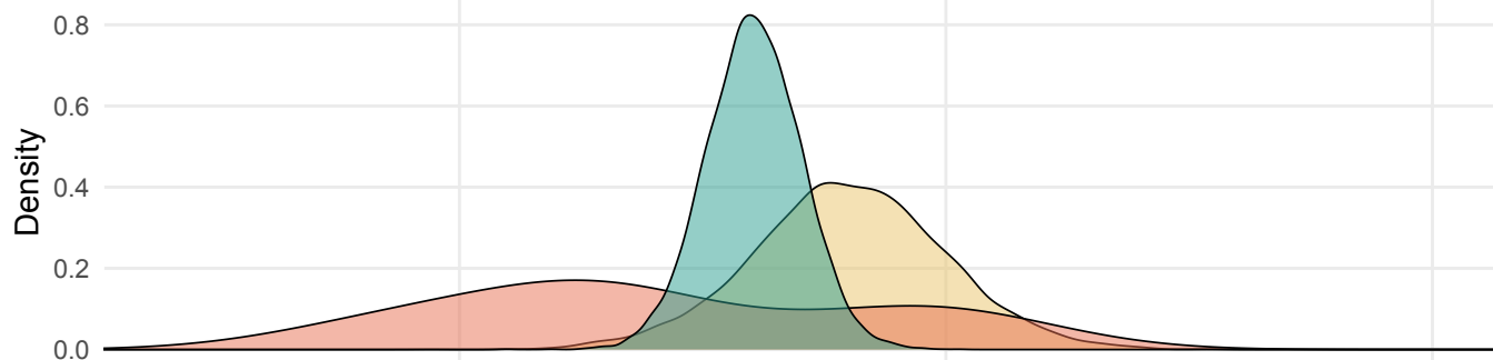
Wide: Normal(0, 6) and Half-normal(6)
