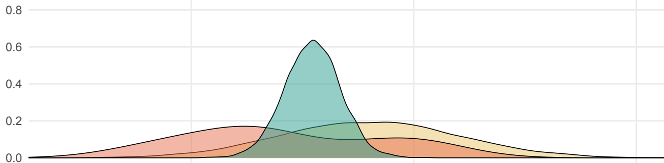
Narrow: Normal(-1, 1) and Half-normal(1)
