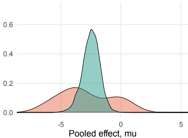
Weak shrinkage: \mu=N(0,100) , \tau=N+(0, 6)
