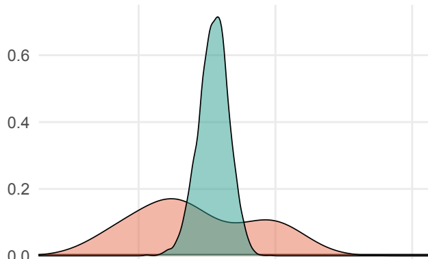
Strong shrinkage: \mu=N(0,100) , \tau=N+(0, 0.67)
