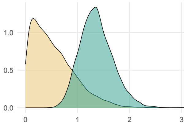
Default shrinkage: \mu=N(0,100) , \tau=N+(0, 2)
