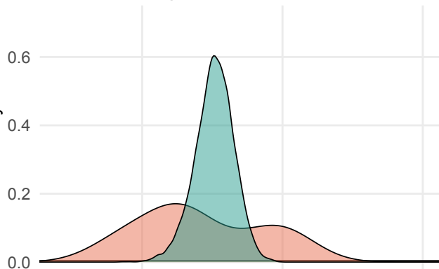
Default shrinkage: \mu=N(0,100) , \tau=N+(0, 2)
