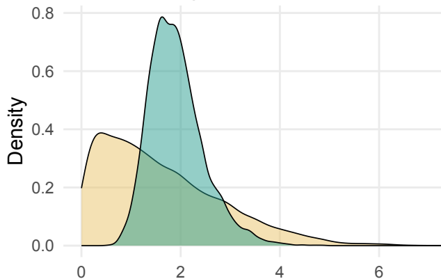
Weak shrinkage: \mu=N(0,100) , \tau=N+(0, 6)
