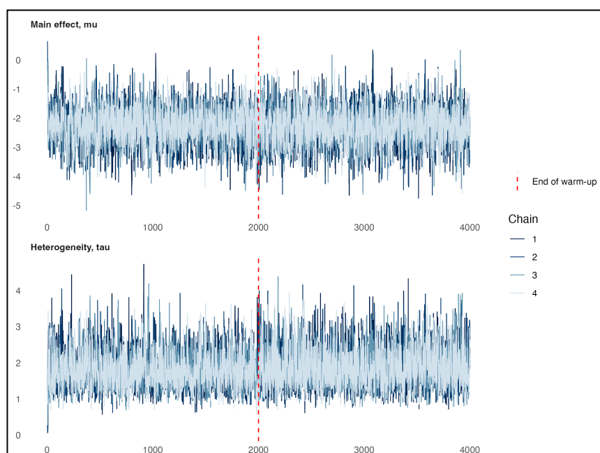
5c) MCMC trace plots for mu and tau
