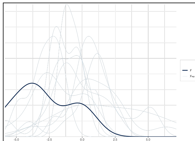
5a) Prior predictive check
