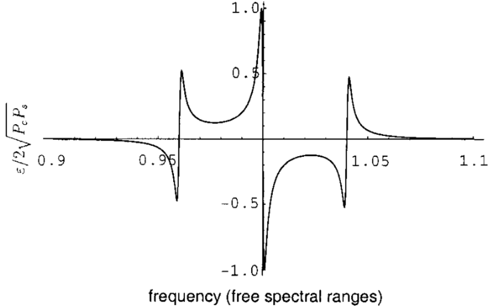
Figure 1.19: Extracted from [3] Typical Pound-Drever-Hall (PDH) error signal obtained by scanning the cavity length across resonance.
