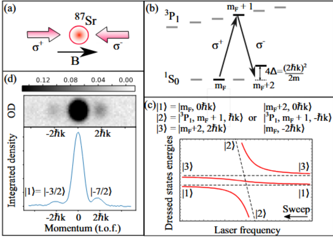
Figure 1.21: Principle of spin-selective detection via coherent momentum transfer ("spin kick"). (a) Counter-propagating beam geometry. (b) Level scheme. (c) Avoided crossing structure for adiabatic transfer. (d) Resulting TOF absorption image showing spatially separated spin components.
