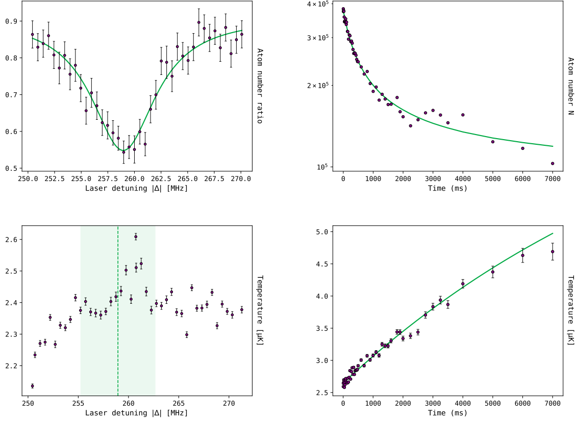
Figure 3.22: Characterization of the molecular line at 259.01 \pm 0.12 MHz in ^{87}\text{Sr} . Top left: resonance spectrum ( I = 19 W/cm 2 , t = 1000 ms), with Lorentzian fit (green). Top right: atom number decay N(t) , fitted via Eq. 3.84 with interpolated T(t) . Bottom left: temperature of the cloud versus detuning; the shaded region and dashed line mark the resonance width and center from the top-left fit. Bottom right: temperature versus illumination time, with a saturating-exponential fit ( \Gamma fixed to the N(t) value). All detunings are measured from the ^{87}\text{Sr} atomic resonance.
