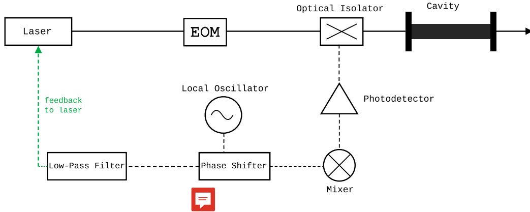
Figure 1.24: Schematic of the Pound-Drever-Hall locking system, extracted and adapted from [6]. The laser is firstly passing through an EOM that is modulating the electric field at frequency f_M , creating two sidebands at frequency f_{\text{laser}} \pm f_M . The carrier at f_{\text{laser}} and the sidebands are passing through the filtering Fabry-Pérot cavity which is reflecting the light going back to the entrance of the cavity. A beamsplitter serving as an optical isolator is reflecting the light to a photodiode. Then this signal is mixed with a local oscillator to extract an error signal to which a low-pass filter is combined to keep only the signal for the locking.
