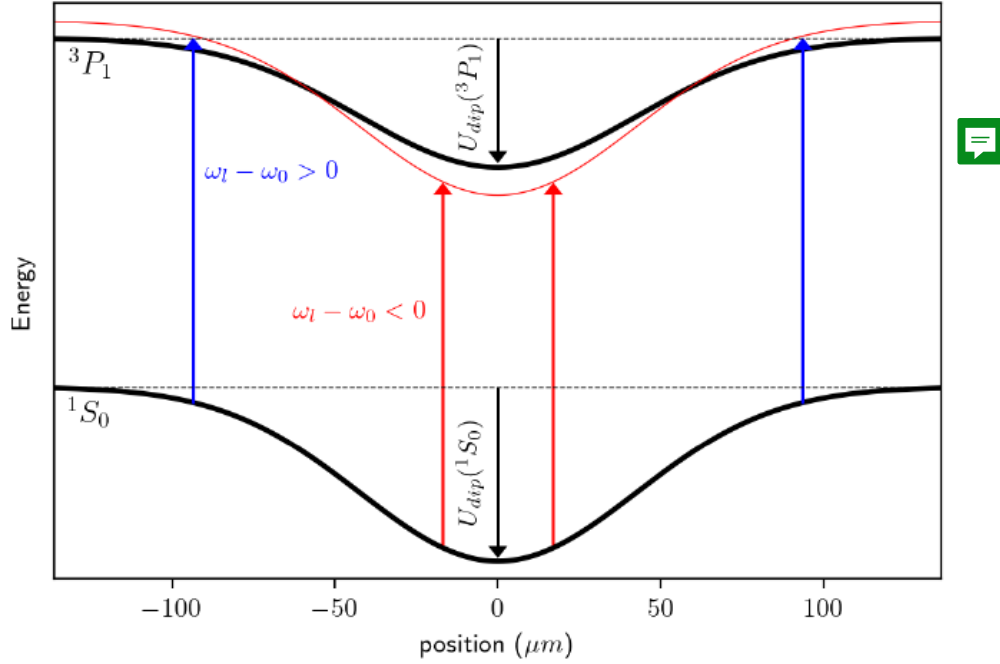
Figure 1.15: Simulation extracted from [4]. Principle of localized 689 nm MOT loading inside the crossed optical dipole trap due to the differential AC Stark shift between ^1S_0 and ^3P_1 .
