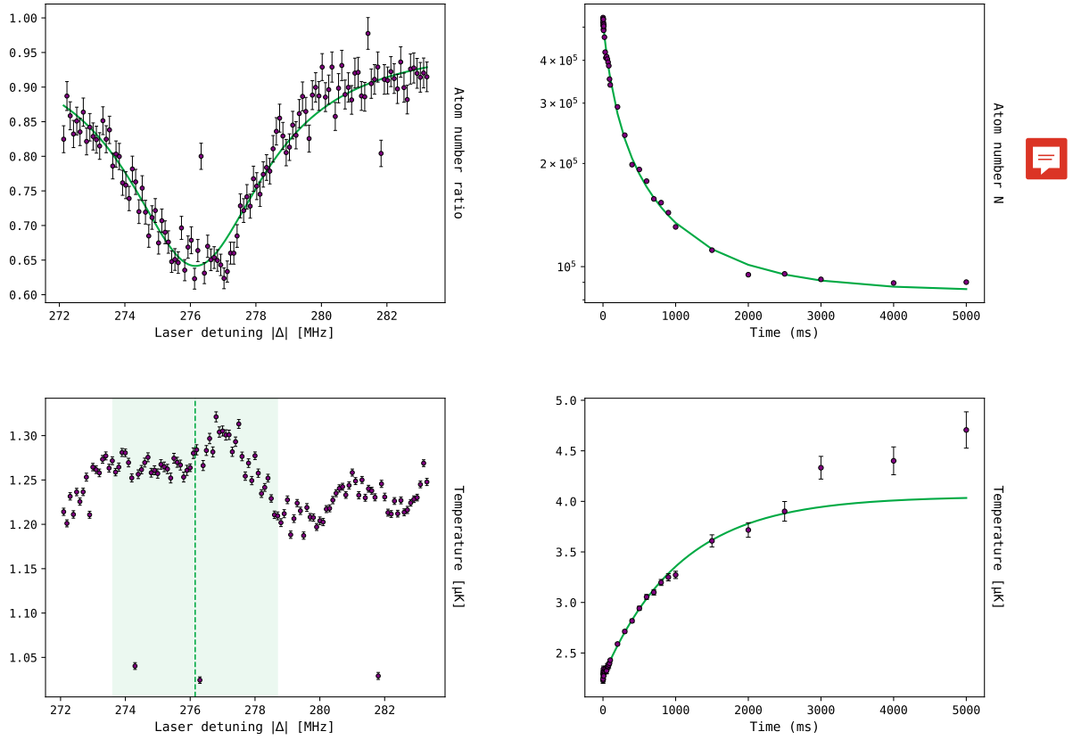
Figure 3.23: Characterization of the molecular line at 276.83 \pm 0.03 MHz in ^{87}\text{Sr} . Panel layout as in Fig. 3.22, with I = 31 W/cm 2 for the N(t)/T(t) fits. All detunings are measured from the ^{87}\text{Sr} atomic resonance.
