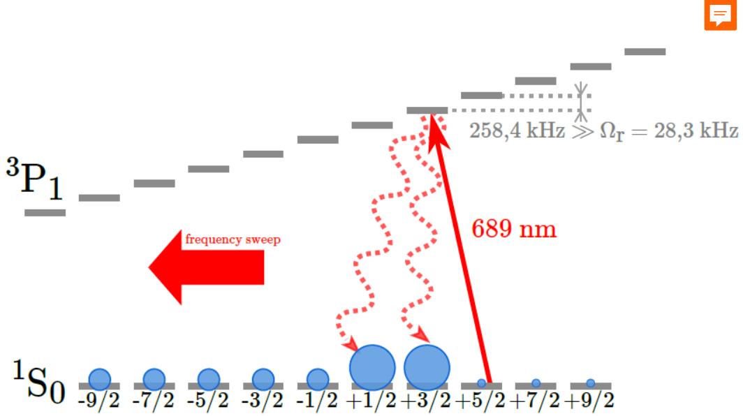
Figure 1.12: Optical pumping scheme on the ^1S_0(F = 9/2) \rightarrow ^3P_1(F = 11/2) transition used to prepare a specific nuclear spin mixture.
