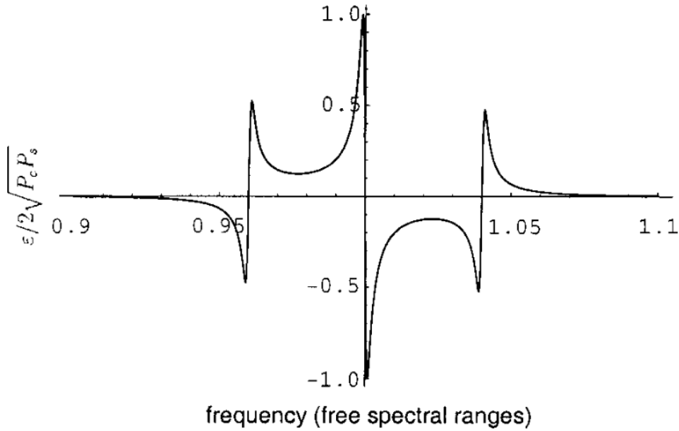
Figure 1.17: Typical Pound-Drever-Hall (PDH) error signal obtained by scanning the cavity length across resonance.
