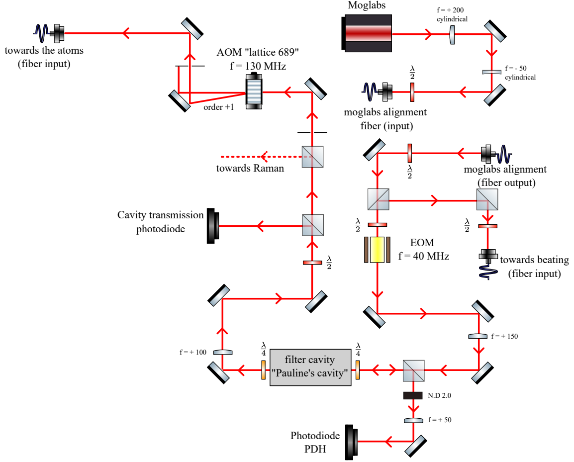
Figure 1.16: Complete optical setup including the Fabry-Pérot cavity and PDH stabilization loop.
