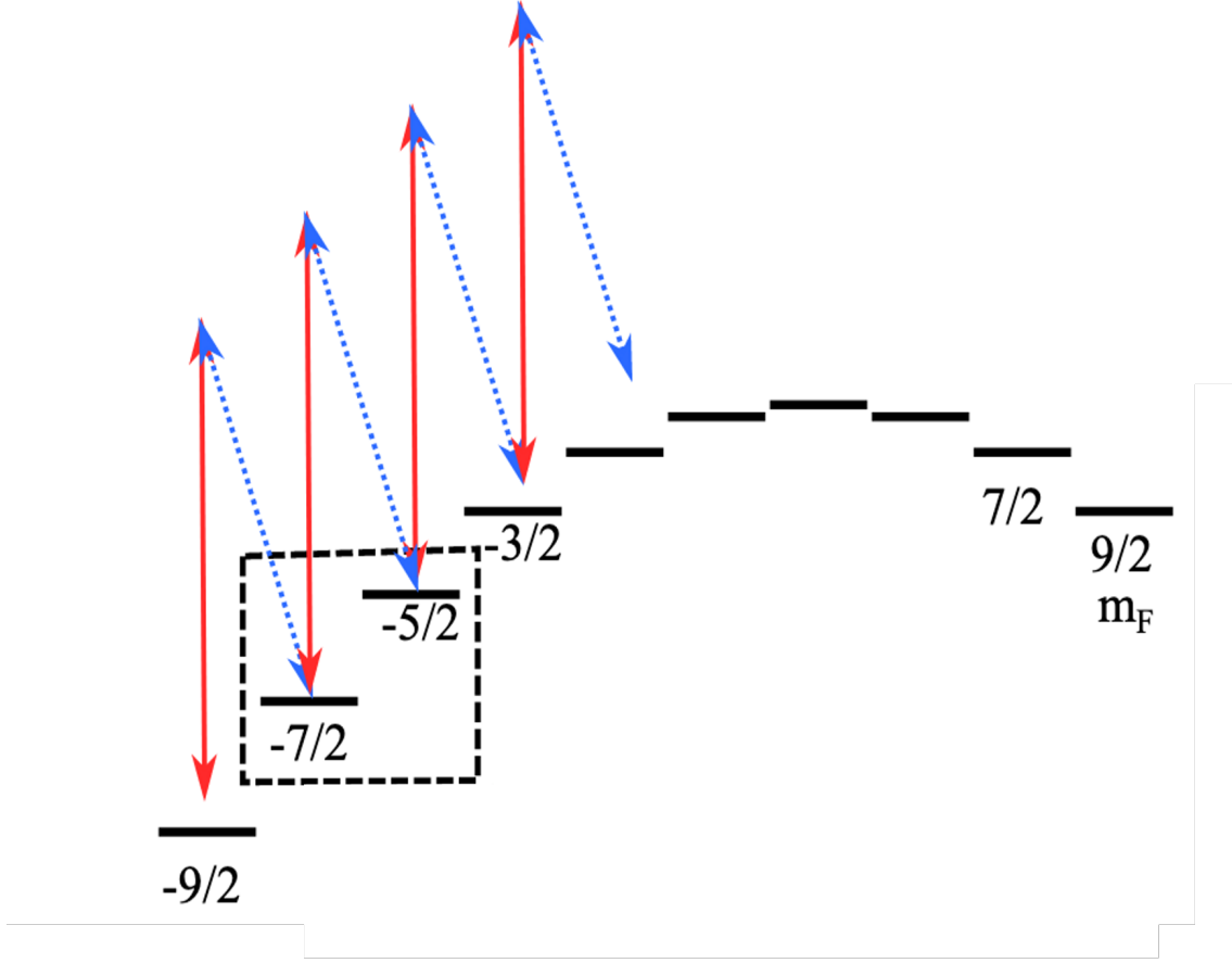
Figure 1.14: Energy level diagram illustrating the Tensorial Light Shift (TLS) and state-selective two-photon Raman transitions.
