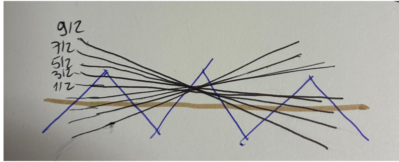
Figure 1.8: Randomization of m_F populations induced by the stirring laser.
