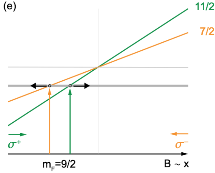
Figure 1.7: Mechanism of population trapping in extreme Zeeman sub-states during the red MOT.
