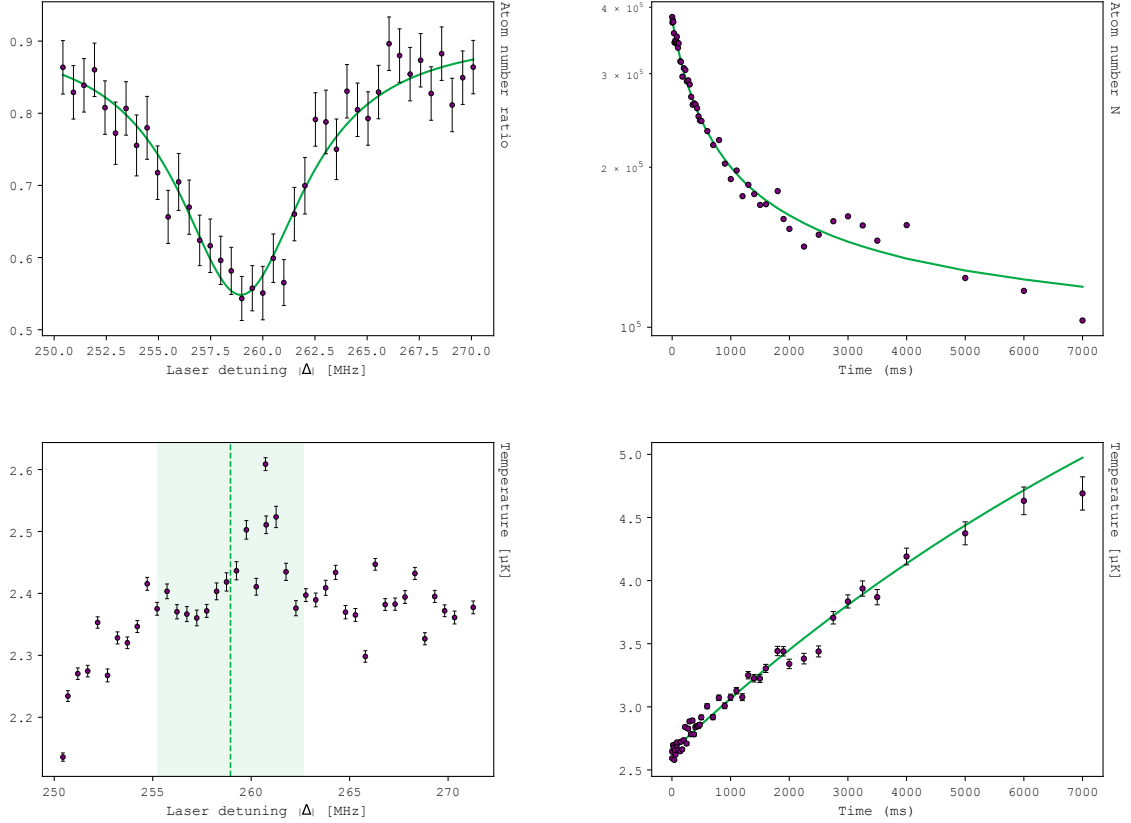
Figure 3.21: Characterization of the molecular line at -259.01 \pm 0.12 MHz in ^{87}\text{Sr} . Top left: resonance spectrum ( I = 19.0 \pm 1.1 \text{ W/cm}^2 , t = 1000 ms, \langle n \rangle = (7.0 \pm 1.0) \times 10^{12} \text{ cm}^{-3} ), with Lorentzian fit (green). Top right: atom number decay N(t) (same intensity and density), fitted via Eq. 3.78 with interpolated T(t) . Bottom left: temperature of the cloud versus detuning; the shaded region and dashed line mark the resonance width and center from the top-left fit. Bottom right: temperature versus illumination time, fitted with the empirical saturating exponential of Eq. 3.93, with the one-body loss rate \Gamma fixed to the value obtained from the fit of N(t) . All detunings are measured from the ^{87}\text{Sr} atomic resonance.
