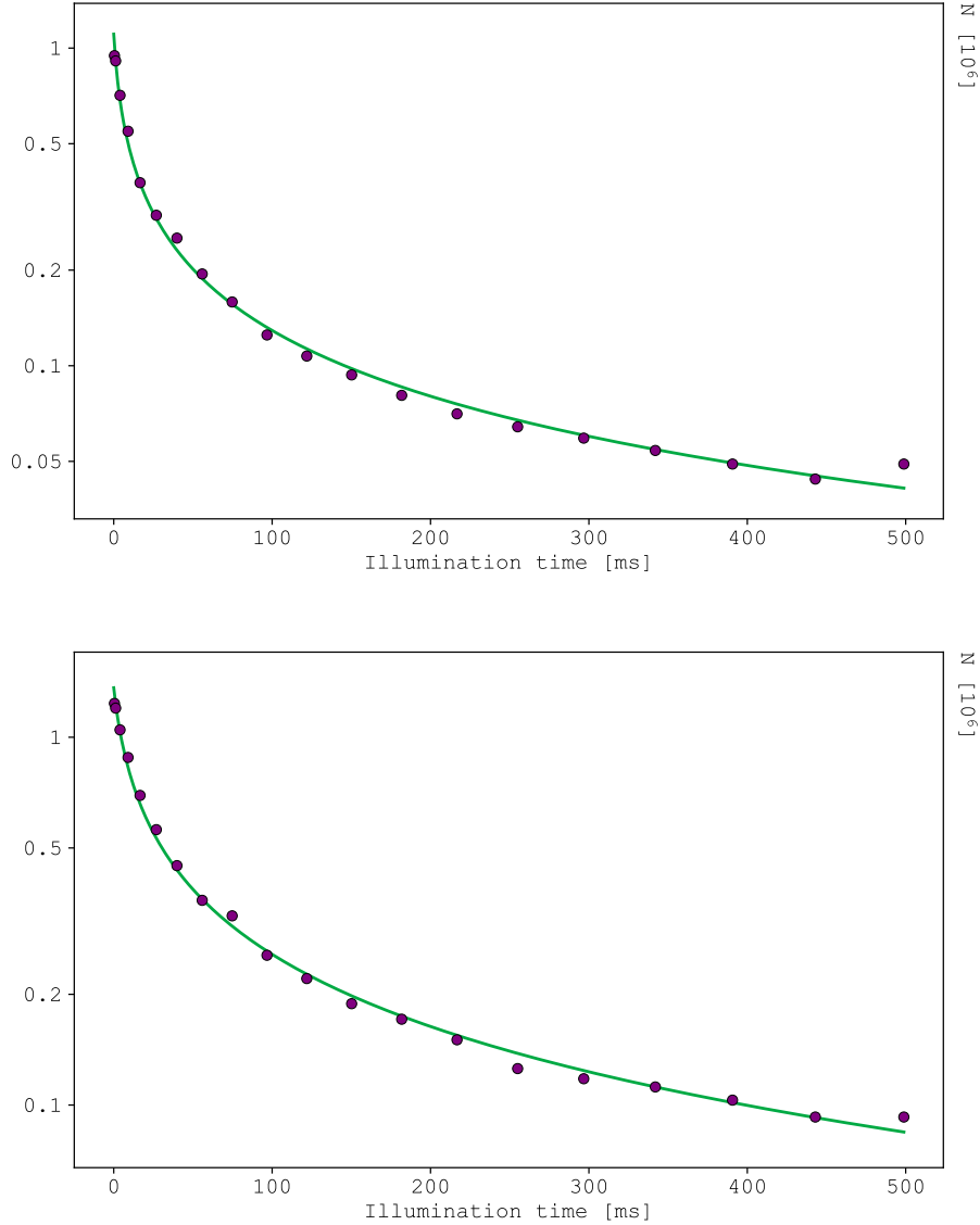
Figure 3.17: Top: atom number decay of ^{88}\text{Sr} on the \nu = -1 line (Fig. 3.13, middle). Bottom: atom number decay on the \nu = -2 line (Fig. 3.13, bottom). Both plots use a logarithmic vertical scale. Solid lines: fit with two-body losses computed locally over the Gaussian density profile, without rethermalization, as expected for the nearly ideal ^{88}\text{Sr} gas [108]. The values of K_2 and l_{\text{opt}} given in the text were obtained with the global fit of the analysis software (Gaussian profile maintained); the local fit shown here gives a value larger by a factor \sim 2 , i.e. the same order of magnitude. Error bars are not shown, as the original raw data could not be recovered.
