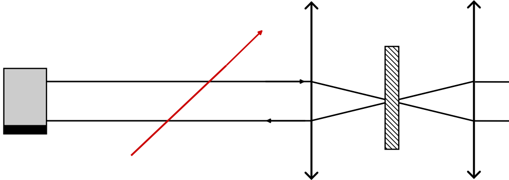
Figure 1.19: MOGlabs External Cavity Diode Laser (ECDL) architecture used for spin manipulation. A diode lasing at 689 nm is frequency settled by an interferential filter marked in red to then be collimated by a lens. The beam is reflected on a second miroir to close a cavity acting as a frequency filter: this system is a cateye. The last lens is used to collimate the beam passing throught an isolater before leaving the laser head.
