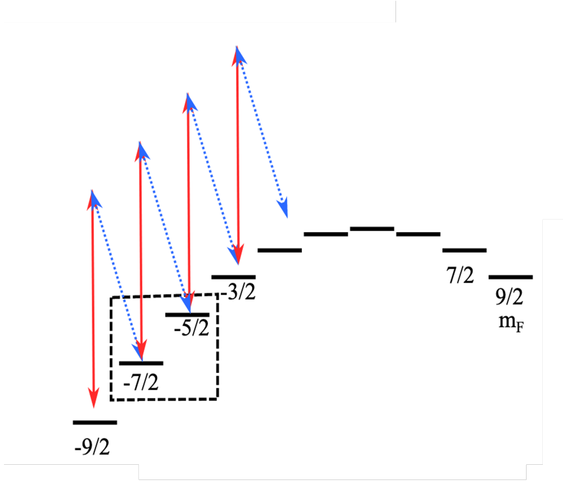
Figure 1.20: Spin manipulation scheme of [5]. The isolation of spin states is allowed by the tensorial shift of the ground states that makes neighbours m_F states isolated from the other resonances.
