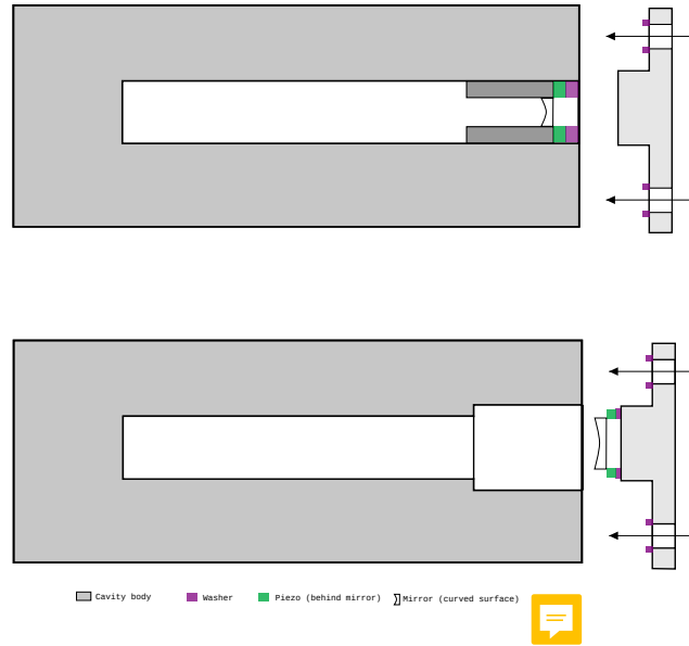
Figure 1.23: Top : Initial fixed cavity assembly using glued mirrors, lacking mechanical alignment degrees of freedom. Bottom : Upgraded and final cavity mount featuring three adjustment screws and compliant washers for precise angular and longitudinal alignment
