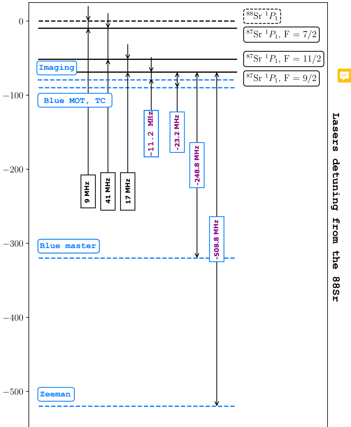
Figure 1.5: Adapted from P.Bataille thesis [1] Diagram of the frequencies of each laser composing the blue chain of the blue MOT broadband cooling. Blue dashed lines indicate the tunable frequencies of the lasers. Plain black lines indicate the transitions of ^{87}\text{Sr} and ^{88}\text{Sr} isotopes.
