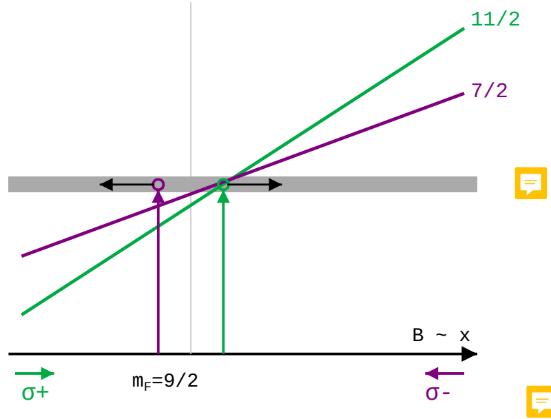
Figure 1.12: (Adapted from [3]) Illustration of the MOT effect on the m_F states of the hyperfine ^3P_1 , F = 11/2 level. The position-dependent light shift brings the two counter-propagating beams into resonance with different m'_F sub-levels ( \sigma^+ with the closed transition to m'_F = 11/2 , \sigma^- with the open transition to m'_F = 7/2 ) at the same position, opening a leak out of the cycling transition.
