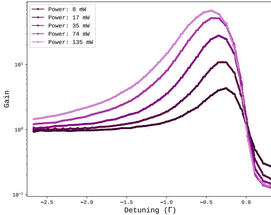
Figure 1.7: Transverse cooling performance as a function of laser detuning and power (adapted from [2]).
