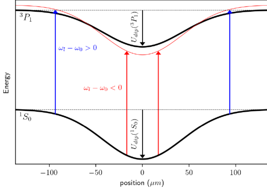
Figure 1.15: Simulation extracted from [4]. Principle of localized 689 nm MOT loading inside the crossed optical dipole trap due to the differential AC Stark shift between ^1S_0 and ^3P_1 .
