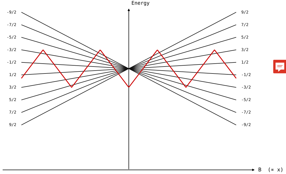
Figure 1.13: (Adapted from [3]) Illustration of the melange concept on the ^1S_0(F = 9/2) \rightarrow ^3P_1(F = 9/2) transition, added to the red MOT cooling to capture extreme spin-state components inaccessible to the counter-propagating lasers of the red MOT.
