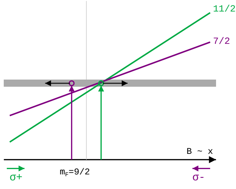
Figure 1.12: (Adapted from [3]) Illustration of the MOT effect on the m_F states of the hyperfine ^3P_1 , F = 11/2 level. The position-dependent light shift brings the two counter-propagating beams into resonance with different m'_F sub-levels ( \sigma^+ with the closed transition to m'_F = 11/2 , \sigma^- with the open transition to m'_F = 7/2 ) at the same position, opening a leak out of the cycling transition.
