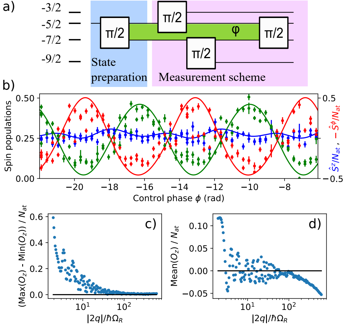
Figure 2.5: Measuring two non-commuting observables in a single realization a) Pulse scheme, highlighting one stage for preparing a well-defined state, and one measurement stage that includes unitary operations before the detection of populations. In frame (b), we monitor, as a function of the control phase, the fractional populations N_{(-7/2, -5/2, -3/2)}/N_{at} , in red, green, and blue, respectively. Error bars reflect only the population measurement uncertainty. Solid lines are the result of simulations of the master equation. We simultaneously acquire N_{-7/2}/N_{at} and N_{-3/2}/N_{at} during the same runs. From N_{-3/2} , we extract an estimate of the projection \langle \hat{s}_{\uparrow, \downarrow}^z \rangle of qubit pseudo-spin, while from N_{-7/2} , we extract an estimate of \langle \hat{s}_{\uparrow, \downarrow}^\phi \rangle , all during the same runs of the experiment. We acquire the population N_{-5/2}/N_{at} by independent runs. The solid lines result from a master equation simulation with a single adjustable parameter: an 18 Hz correction on the linear Zeeman splitting. (c) and (d) present the dependence of \langle \hat{O}_z \rangle on the energy scale separation 2|q|/\hbar\Omega_R for Rabi pulses with a simple square temporal envelope, obtained from numerical simulations. We consider a coherent state with \langle \hat{s}_{\uparrow, \downarrow}^z \rangle = 0 . We take the maximal, minimal, and mean values of \hat{O}_z over a 2\pi variation of the control phase. We operate our experiment at 2|q|/\hbar\Omega_R \simeq 9 , providing the best balance between technically-limited decoherence and scheme fidelity.
