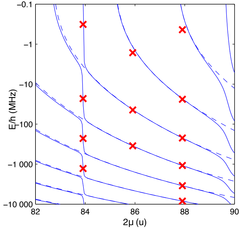
Figure 3.7: This graph - extracted from [88]- confronts the experimental internal states in red crosses to their theoretical predictions for different reduced mass of strontium isotopes. The theoretical model guarantees approximated scales for molecular lines of ^{87}\text{Sr} but not precisely because this model neglects the hyperfine interaction of the species.
