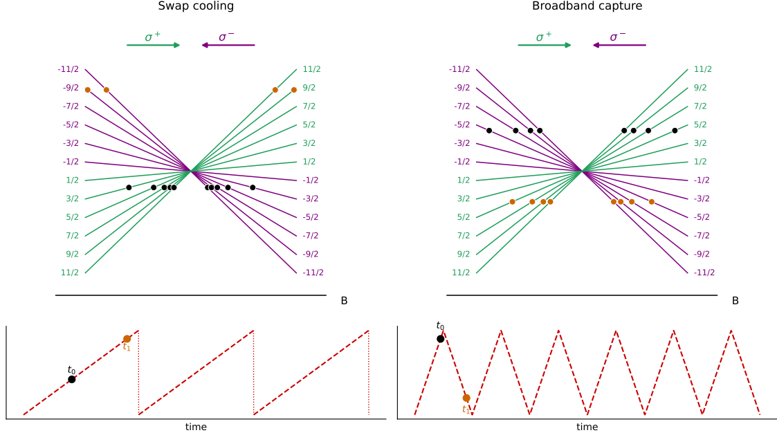
Figure 1.14: Sequential stages of the 689 nm red MOT. From left to right : swap cooling and broadband capture (adapted from [31]). The size of the cloud is decreasing with the cooling since the atoms are kicked in the opposite direction of the resonant laser of right polarization.
