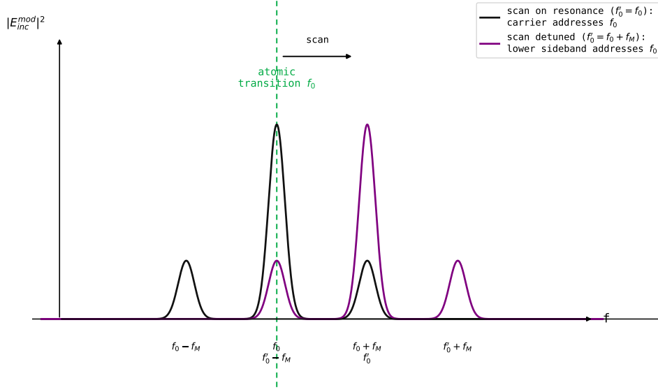
Figure 3.12: Scheme of the PDH sidebands addressing the atomic resonance, shown at two snapshots of the laser frequency scan. The atomic transition sits at the fixed frequency f_0 (green dashed line). In black: the carrier is scanned onto resonance ( f'_0 = f_0 ), producing the true photoassociation signal. In purple: the carrier is instead detuned to f'_0 = f_0 + f_M , so that it is itself off-resonance, but its lower sideband coincides with f_0 and drives a spurious ("ghost") loss resonance. As the scan sweeps f'_0 , this coincidence recurs whenever f'_0 = f_0 \pm f_M , producing satellite peaks such as the one reported in Fig. 3.13.
