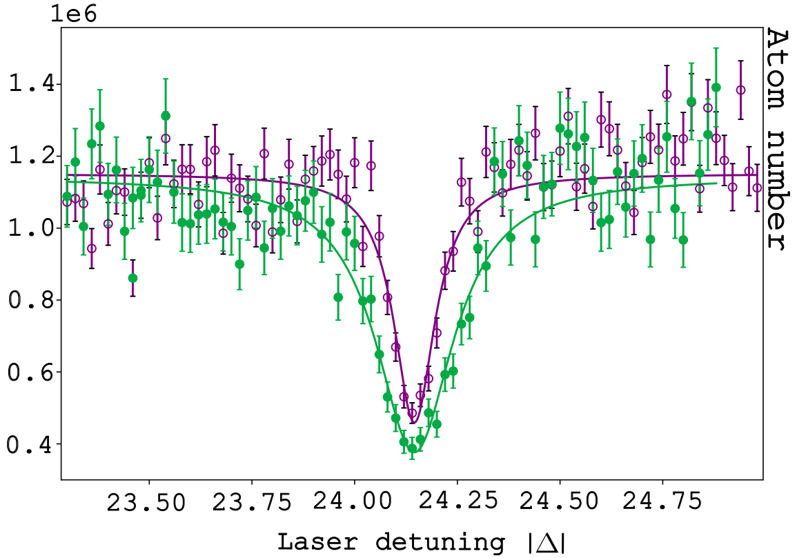
Figure 3.14: Comparison of the \nu = -1 molecular line profile with two different sources. The MOGlabs dataset (green) yields a line about twice as broad as the stable injection locked laser source (purple).
