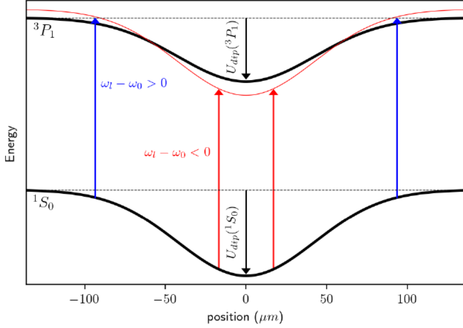
Figure 1.15: Simulation extracted from [21]. Principle of localized 689 nm MOT loading inside the crossed optical dipole trap due to the differential AC Stark shift between ^1S_0 and ^3P_1 .
