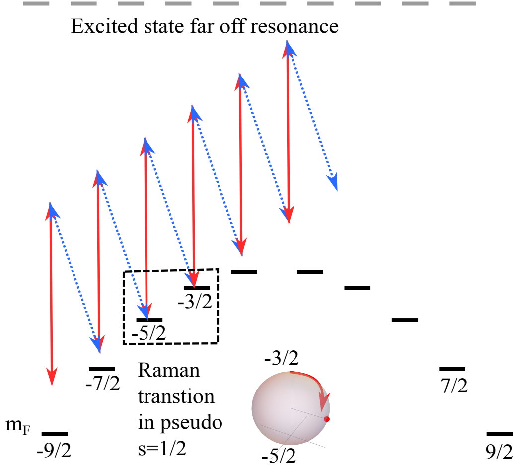
Figure 1.20: Spin manipulation scheme of [22]. The isolation of spin states is allowed by the tensorial shift of the ground states that makes neighbours m_F states isolated from the other resonances.
