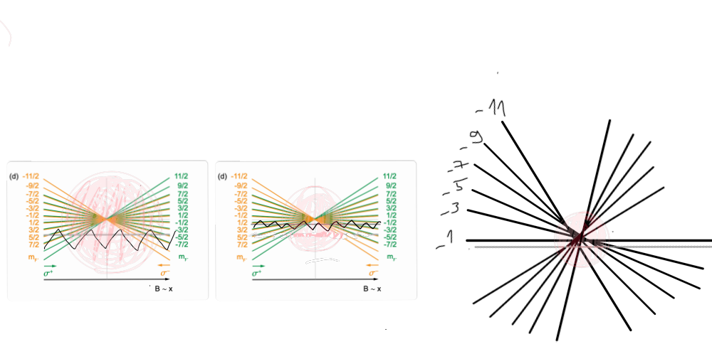
Figure 1.10: Sequential stages of the 689 nm red MOT: broadband capture, compression, and single-frequency cooling (adapted from [? ]).
