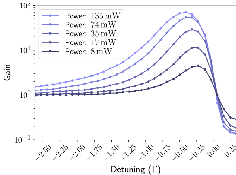
Figure 1.4: Transverse cooling performance as a function of laser detuning and power (adapted from [?]).
