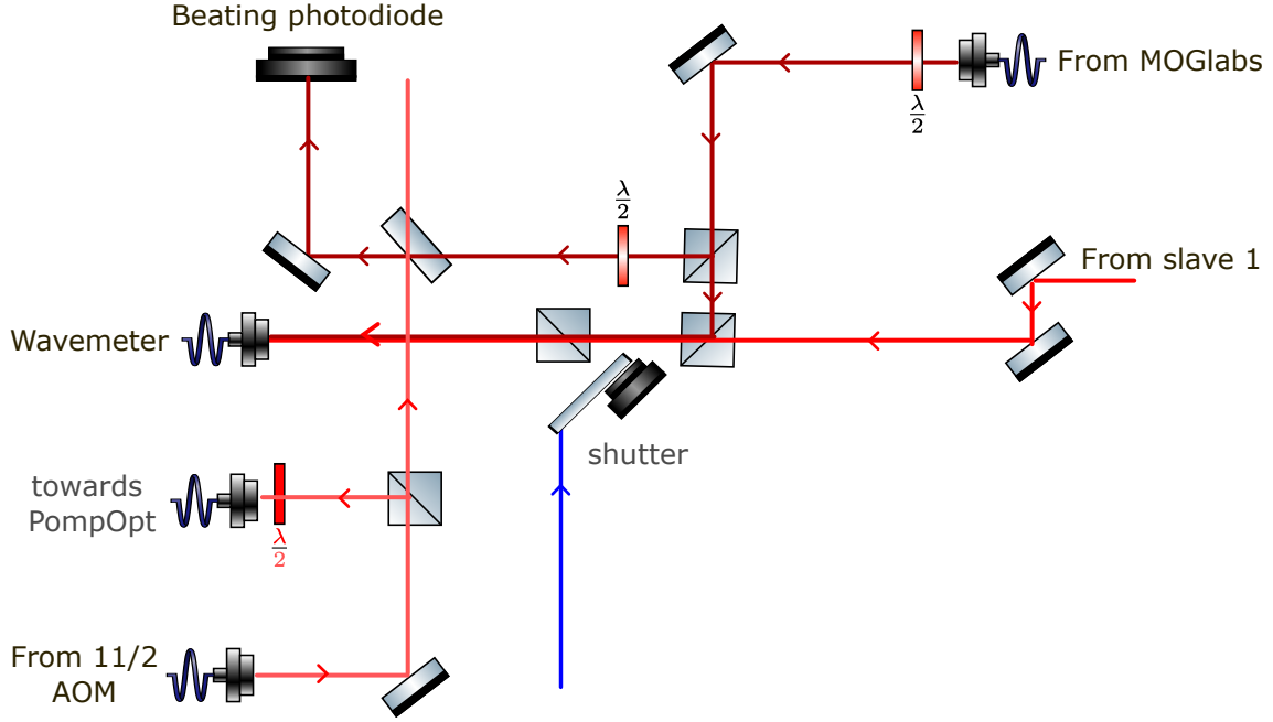
Figure 3.8: Beating scheme for PA process between the light from "AOM 11/2" and MOGlabs. The light is coming from ?? to split in two arms: optical pumping and PA. This last one serves for MOGlabs locking in a beating procedure where the beam is recombined by the 50/50 waveplate superposing with slave 1 beam.
