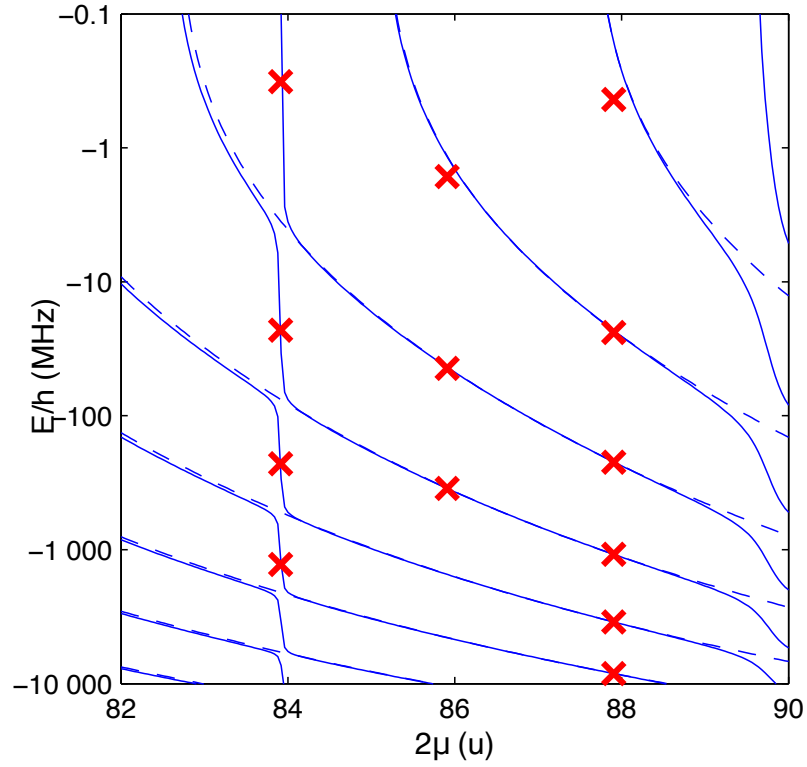
Figure 3.7: This graph - extracted from [?] - confronts the experimental internal states in red crosses to their theoretical predictions for different reduced mass of strontium isotopes. The theoretical model guarantees approximated scales for molecular lines of ^{87}\text{Sr} but not precisely because this model neglects the hyperfine interaction of the species.
