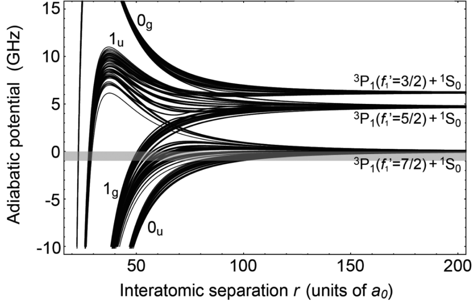
Figure 3.5: Density of molecular potentials for ^{173}\text{Yb} with three hyperfine states inhancing numerous triplet of quantum numbers (T, F, R) . The spectral lines are identified by S_{u/g} with S the total orbital momentum of the molecule and u/g the parity of the electronic wavefunction (see ??).
