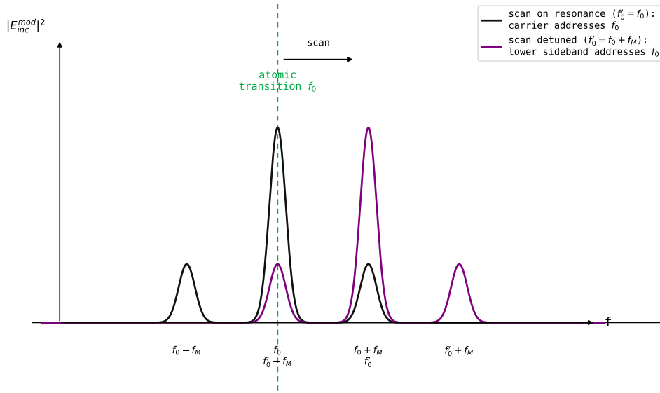
Figure 3.11: Scheme of the PDH sidebands addressing the atomic resonance, shown at two moments of the laser frequency scan. The atomic transition is at the fixed frequency f_0 (green dashed line). In black: the carrier is scanned onto resonance ( f'_0 = f_0 ), giving the true signal. In purple: the carrier is detuned to f'_0 = f_0 + f_M , so that it is itself off resonance, but its lower sideband coincides with f_0 and drives a parasitic ("ghost") loss resonance. During the scan, this happens again whenever f'_0 = f_0 \pm f_M , giving satellite peaks such as the one of Fig. 3.12.
