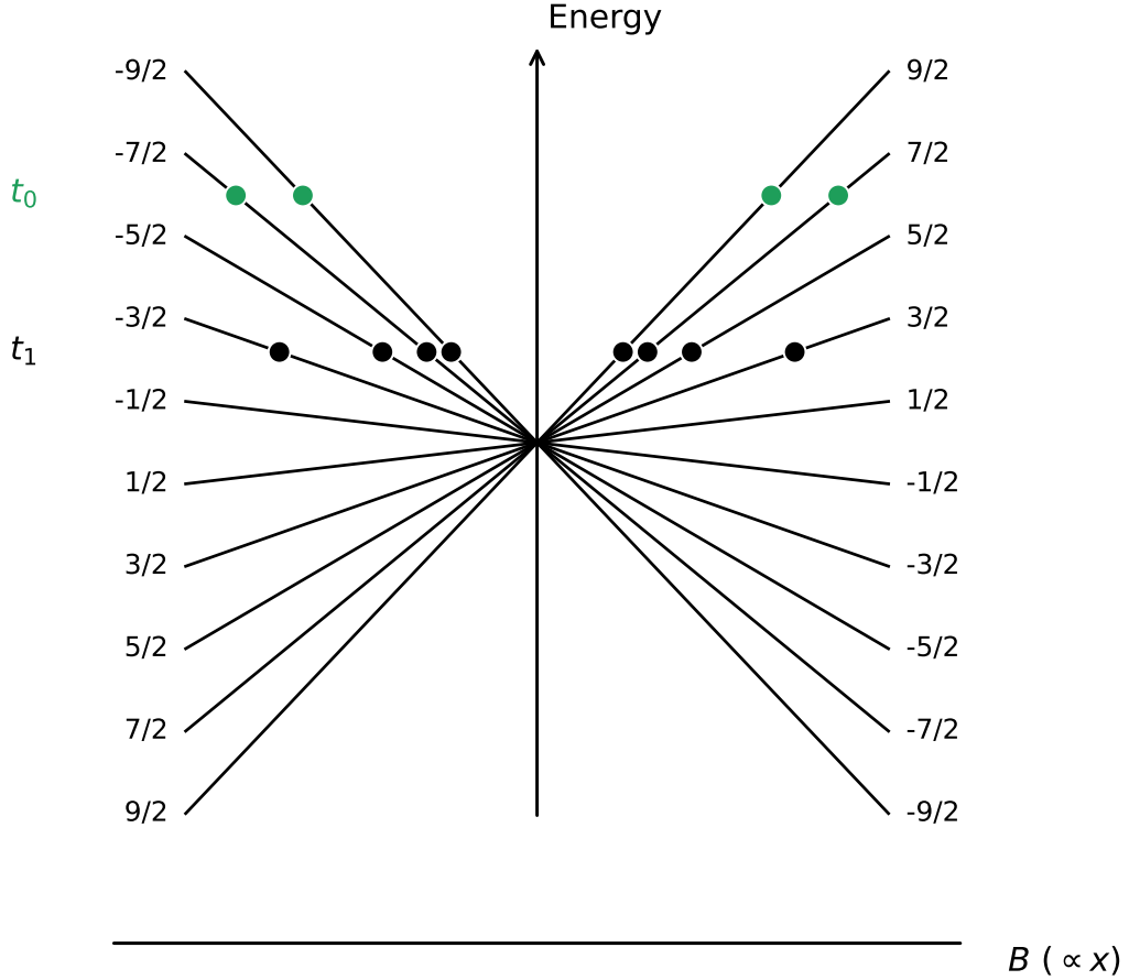
Figure 1.15: Spatial dependence of the resonance condition on each m_F sub-level, as a function of position x ( B \propto x ) – adapted from the principle illustrated in Fig. 2.8(d) of [31].
