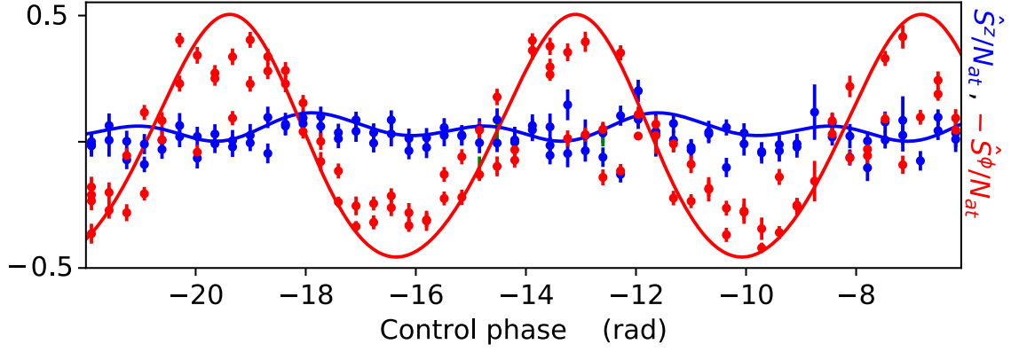
Figure 2.5: Measuring two non-commuting observables in a single realization a) Pulse scheme, highlighting one stage for preparing a well-defined state, and one measurement stage that includes unitary operations before the detection of populations. In frame (b), we monitor, as a function of the control phase, the fractional populations N_{(-7/2, -5/2, -3/2)}/N_{at} , in red, green, and blue, respectively. Error bars reflect only the population measurement uncertainty. Solid lines are the result of simulations of the master equation. We simultaneously acquire N_{-7/2}/N_{at} and N_{-3/2}/N_{at} during the same runs. From N_{-3/2} , we extract an estimate of the projection \langle \hat{s}_{\uparrow, \downarrow}^z \rangle of qubit pseudo-spin, while from N_{-7/2} , we extract an estimate of \langle \hat{s}_{\uparrow, \downarrow}^\phi \rangle , all during the same runs of the experiment. We acquire the population N_{-5/2}/N_{at} by independent runs. The solid lines result from a master equation simulation with a single adjustable parameter: an 18 Hz correction on the linear Zeeman splitting. (c) and (d) present the dependence of \langle \hat{O}_z \rangle on the energy scale separation 2|q|/\hbar\Omega_R for Rabi pulses with a simple square temporal envelope, obtained from numerical simulations. We consider a coherent state with \langle \hat{s}_{\uparrow, \downarrow}^z \rangle = 0 . We take the maximal, minimal, and mean values of \hat{O}_z over a 2\pi variation of the control phase. We operate our experiment at 2|q|/\hbar\Omega_R \simeq 9 , providing the best balance between technically-limited decoherence and scheme fidelity.
