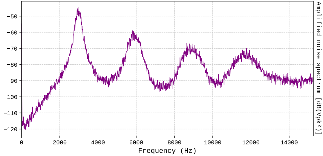
Figure 1.27: Closed-loop noise spectrum measured with the Red Pitaya, showing the servo bump at 3 kHz and its multiples.
