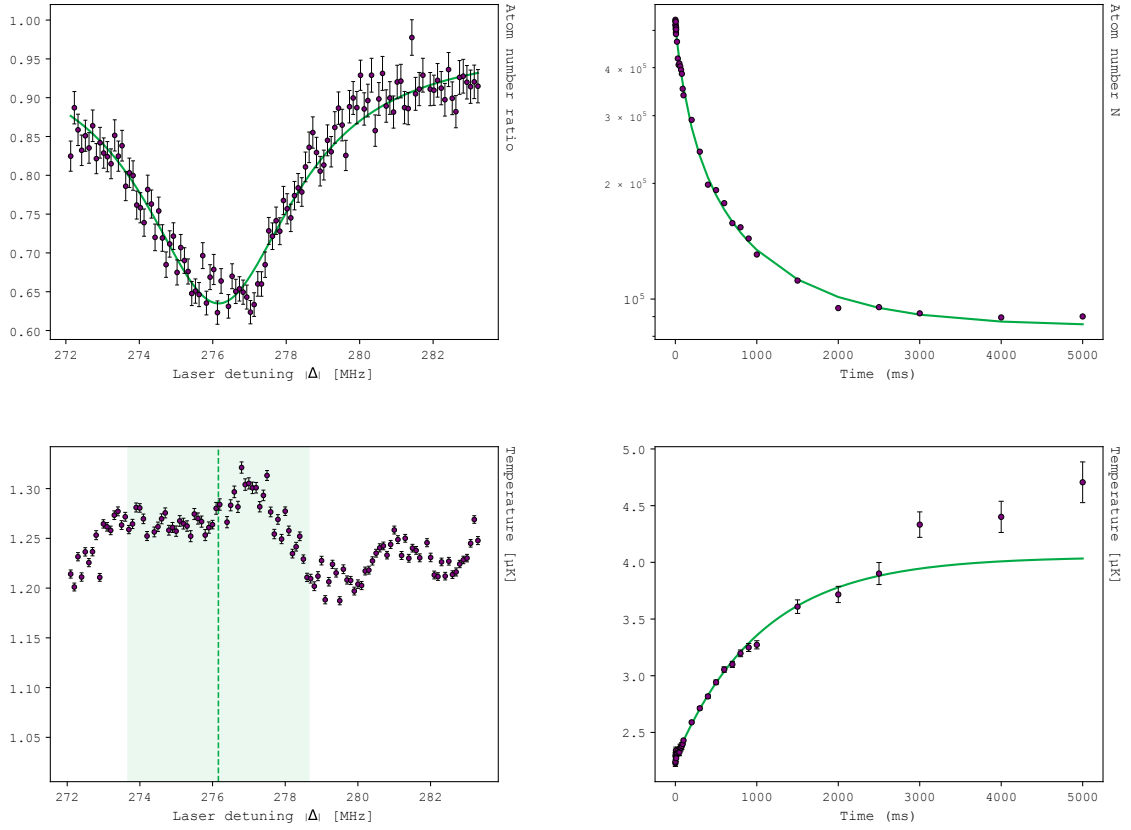
Figure 3.22: Characterization of the molecular line at -276.83 \pm 0.03 MHz in ^{87}\text{Sr} . Panel layout as in Fig. 3.21, with I = 5.2 \pm 0.3 W/cm ^2 for the spectrum and I = 31.0 \pm 1.8 W/cm ^2 for the N(t)/T(t) fits, and \langle n \rangle = (1.6 \pm 0.2) \times 10^{13} cm ^{-3} (spectrum) and (7.8 \pm 1.1) \times 10^{12} cm ^{-3} (decay). Brought to the same intensity and density ( K_2 \propto I ), the loss at the line center after 1 s in the spectrum ( (60 \pm 5)\% expected) is compatible within 2\sigma with the one of the decay once the non-molecular PA-induced loss is removed ( (69 \pm 3)\% at 1 s, (74 \pm 2)\% raw). All detunings are measured from the ^{87}\text{Sr} atomic resonance.
