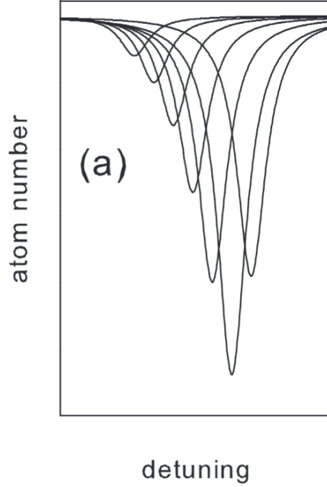
Figure 1.4: Illustration of Doppler cooling: velocity classes are shifted relative to the atomic resonance frequency \omega_0 .
