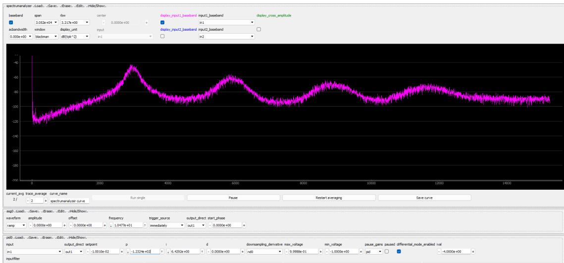
Figure 1.26: Closed-loop noise analysis and mechanical resonance identification using the Red Pitaya.
