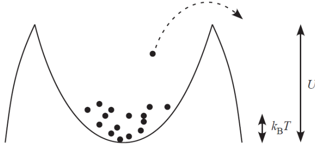
Figure 1.14: Evaporative cooling mechanism in an inclined crossed optical dipole trap, illustrating the escape of high-energy atoms and subsequent re-thermalization.
