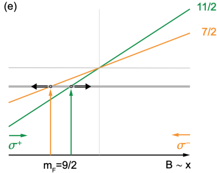
Figure 1.10: Mechanism of population trapping in extreme Zeeman sub-states during the red MOT.
