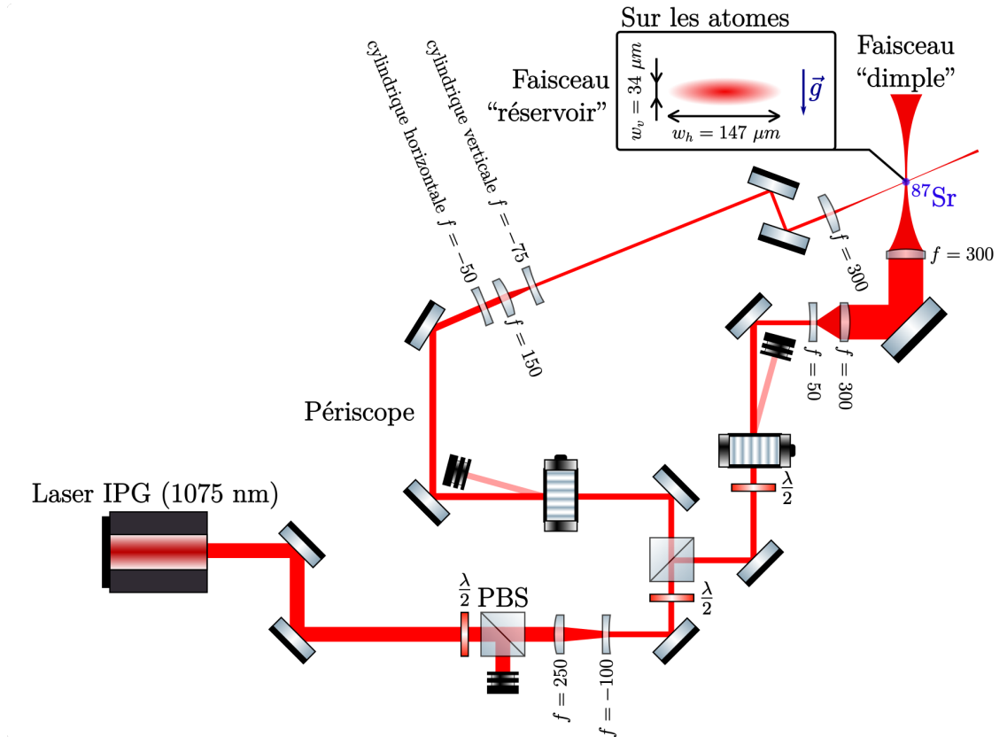
Figure 1.15: Optical layout of the 1075 nm crossed dipole trap laser system.
