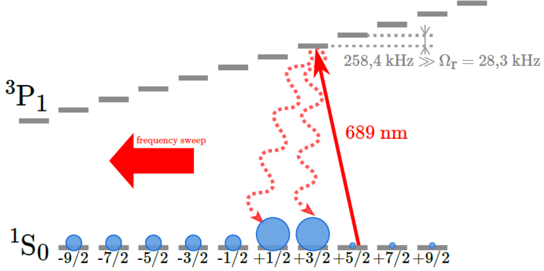
Figure 1.16: Optical pumping scheme on the ^1S_0(F = 9/2) \rightarrow ^3P_1(F = 11/2) transition used to prepare a specific nuclear spin mixture.
