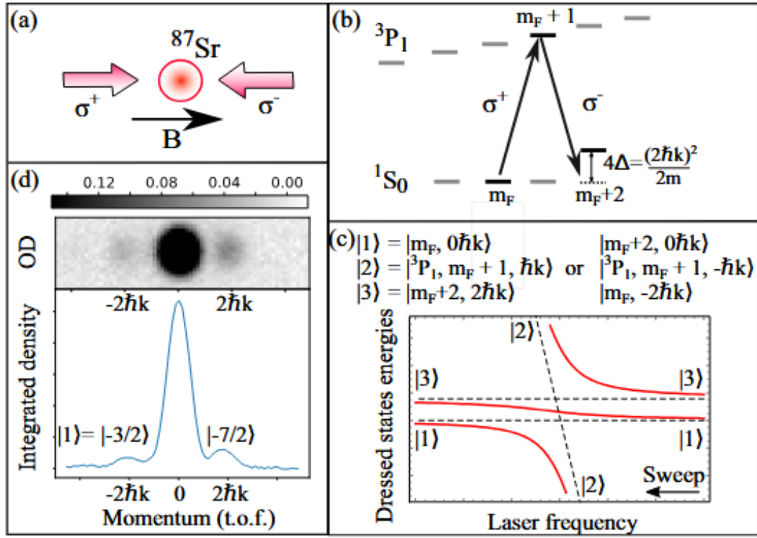
Figure 1.27: Principle of spin-selective detection via coherent momentum transfer ("spin kick"). (a) Counter-propagating beam geometry. (b) Level scheme. (c) Avoided crossing structure for adiabatic transfer. (d) Resulting TOF absorption image showing spatially separated spin components.
