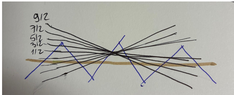
Figure 1.11: Randomization of m_F populations induced by the 689 nm stirring laser.
