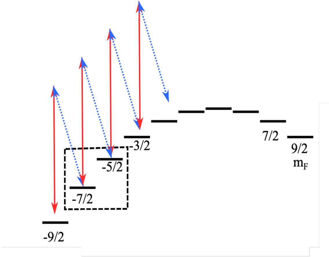
Figure 1.20: Spin manipulation scheme of [4]. The isolation of spin states is allowed by the tensorial shift of the ground states that makes neighbours m_F states isolated from the other resonances.
