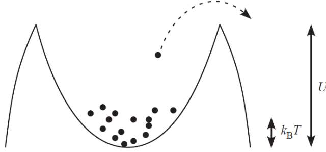
Figure 1.16: Evaporative cooling mechanism in a crossed optical dipole trap, illustrating the escape of high-energy atoms and subsequent re-thermalization.
