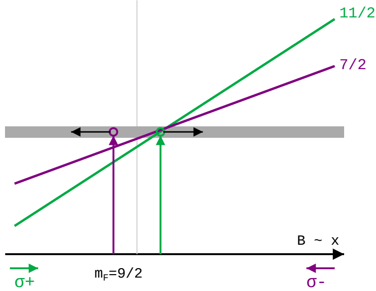
Figure 1.14: (Adapted from [31]) Illustration of the MOT effect on the m_F states of the hyperfine ^3P_1 , F = 11/2 level. The position-dependent Zeeman shift brings the two counter-propagating beams into resonance with different m'_F sub-levels ( \sigma^+ with the closed transition to m'_F = 11/2 , \sigma^- with the open transition to m'_F = 7/2 ) at the same position. The imbalance between the two processes, set by their Clebsch-Gordan coefficients, still favors restoring trapping locally (see text); the actual loss mechanism is discussed below.
