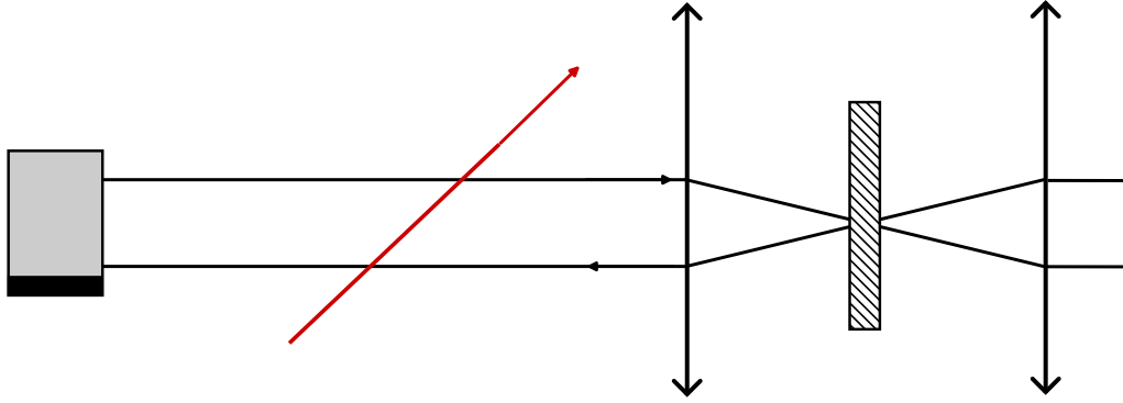
Figure 1.19: MOGlabs External Cavity Diode Laser (ECDL) architecture used for spin manipulation. A diode lasing at 689 nm is frequency settled by an interferential filter marked in red to then be collimated by a lens. The beam is reflected on a second miroir to close a cavity acting as a frequency filter: this system is a cateye. The last lens is used to collimate the beam passing throught an isolater before leaving the laser head.
