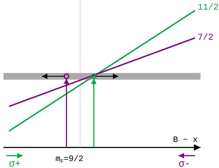
Figure 1.12: (Adapted from [30]) Illustration of the MOT effect on the m_F states of the hyperfine ^3P_1, F = 11/2 level. The position-dependent Zeeman shift brings the two counter-propagating beams into resonance with different m_F' sub-levels ( \sigma^+ with the closed transition to m_F' = 11/2 , \sigma^- with the open transition to m_F' = 7/2 ) at the same position. The imbalance between the two processes, set by their Clebsch-Gordan coefficients, still favors restoring trapping locally (see text); the actual loss mechanism is discussed below.
