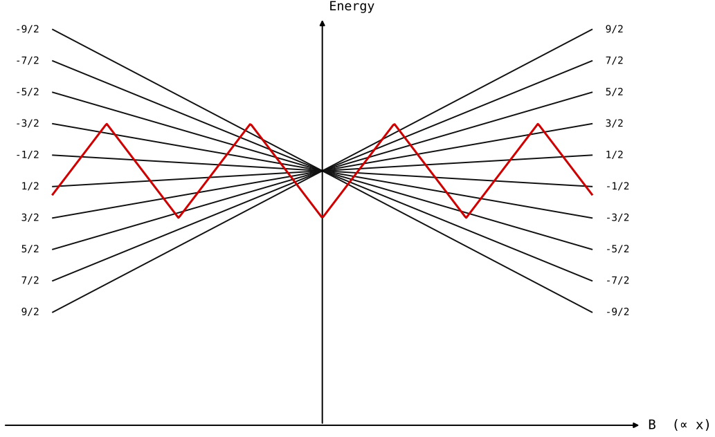
Figure 1.13: Illustration of the melange concept on the ^1S_0(F = 9/2) \rightarrow ^3P_1(F = 9/2) transition, added to the red MOT cooling to capture extreme spin-state components inaccessible to the counter-propagating lasers of the red MOT. Left: spatial dependence of the resonance condition on each m_F sub-level, as a function of position x ( B \propto x ). Right: the stirring laser's frequency, swept in a sawtooth pattern over time . At each instant t_0 , the instantaneous frequency (right) is simultaneously resonant with several (m_F, x) pairs (left, black dots); sweeping this frequency over time thus randomizes the m_F population across the whole trap.
