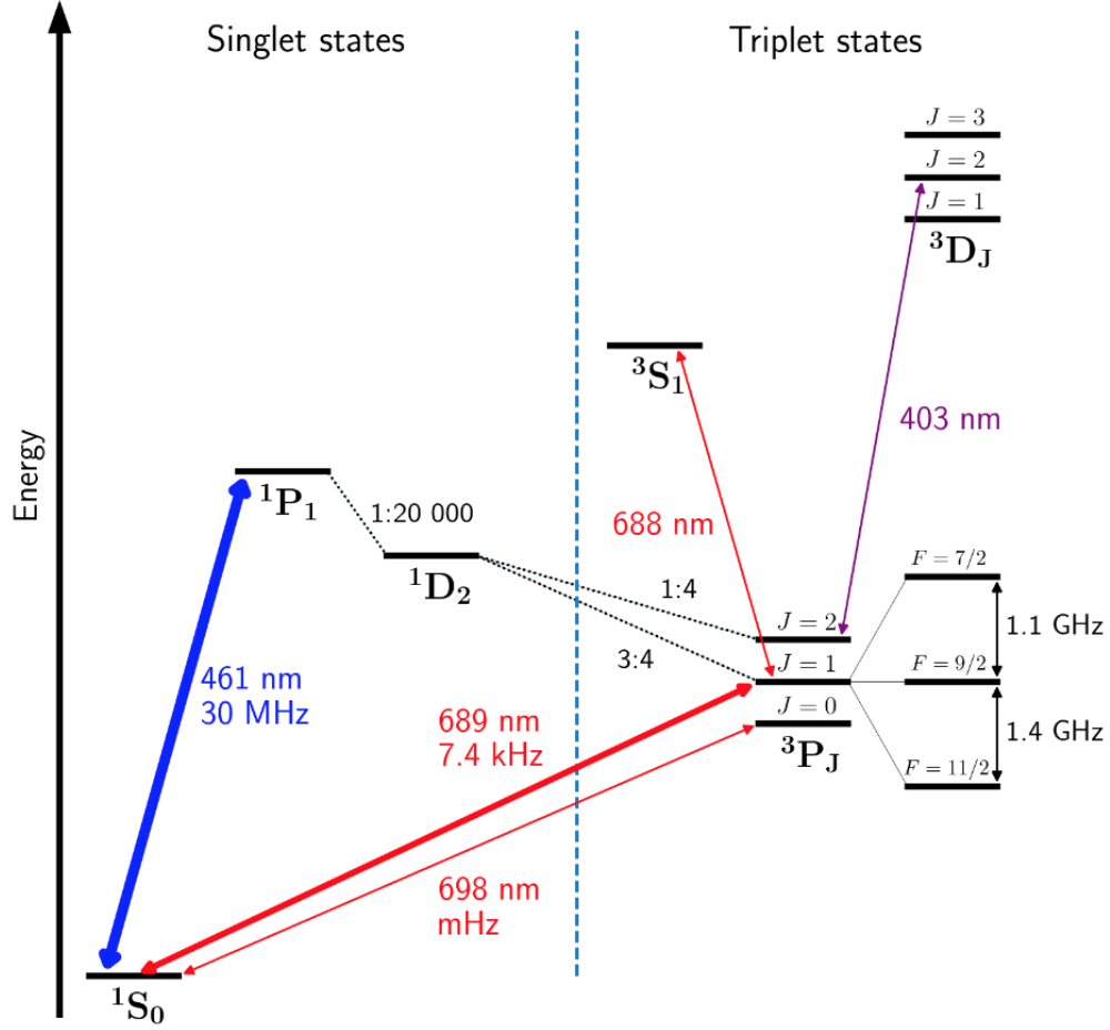
Figure 1.1: Extracted from [2] Energy spectrum of ^{87}\text{Sr} including fine and hyperfine interactions. In blue the 461 nm transition used for TC, Zeeman cooling, blue MOT stage and imaging. The purple arrow indicates the repump line at 403 nm from the metastable state ^3P_2 used for the atoms leaking from the intermediate ^1D_2 state. In red the transition to ^3P_1 at 689 nm used for all stages of the red MOT, optical pumping, spin manipulation, coherent manipulation (see Chap.2), photoassociation (see Chap.3, through the different hyperfine states F = 7/2, 9/2, 11/2 ). The 698 nm transition indicates the clock transition which we do not use in this experiment.
