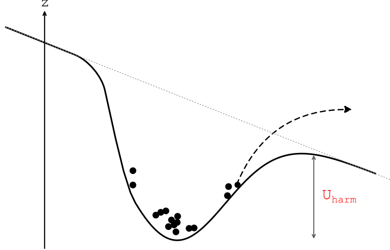
Figure 1.16: Evaporative cooling mechanism in a crossed optical dipole trap, illustrating the escape of high-energy atoms and subsequent re-thermalization.
