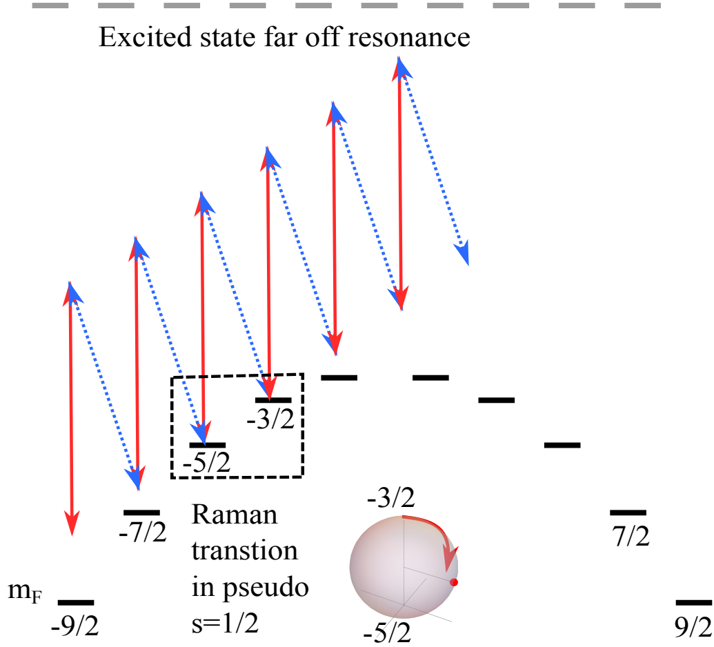
Figure 1.20: Spin manipulation scheme of [1]. The isolation of spin states is allowed by the tensorial shift of the ground states that makes neighbours m_F states isolated from the other resonances.
