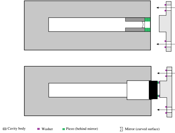
Figure 1.23: Top : Initial fixed cavity assembly using glued mirrors, lacking mechanical alignment degrees of freedom. Bottom : Upgraded and final cavity mount featuring three adjustment screws and compliant washers for precise angular and longitudinal alignment
