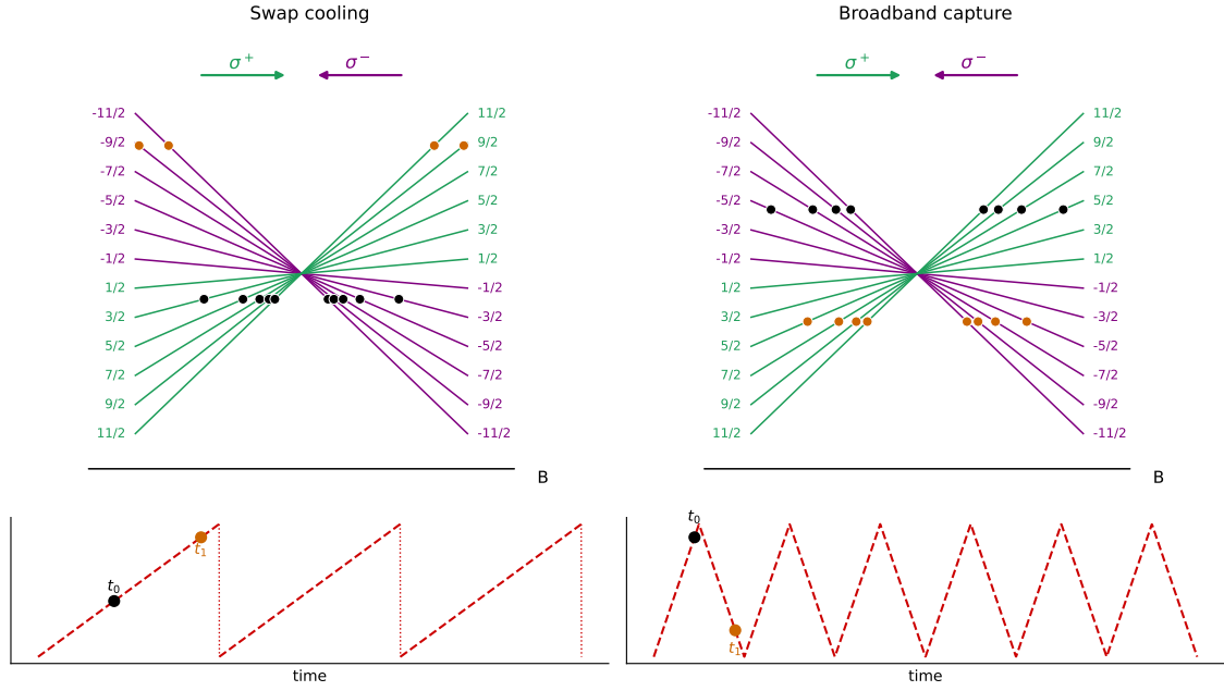
Figure 1.14: Sequential stages of the 689 nm red MOT. From left to right : swap cooling and broadband capture (adapted from [31]). The size of the cloud is decreasing with the cooling since the atoms are kicked in the opposite direction of the resonant laser of right polarization.
