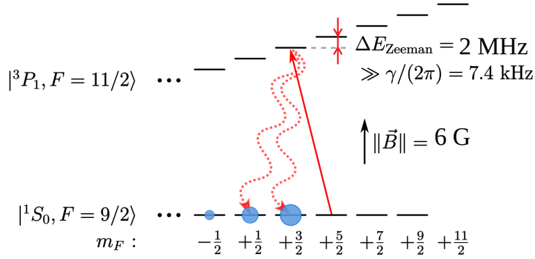
Figure 1.18: Extracted from [1] Optical pumping scheme on the ^1S_0(F = 9/2) \rightarrow ^3P_1(F = 11/2) transition used to prepare a specific nuclear spin mixture. The red laser is ramped through the target energy level of ^3P_1 : the atoms decay to neighbours states m_F \pm 1 of ^1S_0
