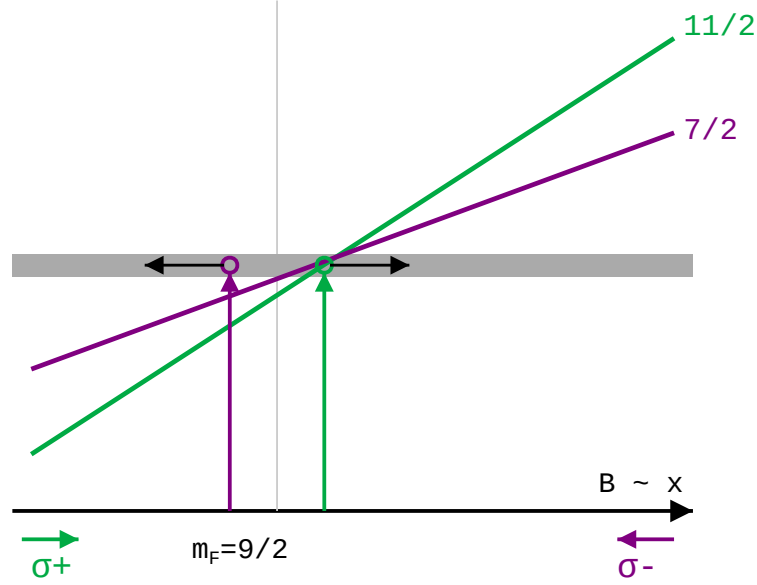
Figure 1.12: (Adapted from [31]) Illustration of the MOT effect on the m_F states of the hyperfine ^3P_1, F = 11/2 level. The position-dependent Zeeman shift brings the two counter-propagating beams into resonance with different m'_F sub-levels ( \sigma^+ with the closed transition to m'_F = 11/2 , \sigma^- with the open transition to m'_F = 7/2 ) at the same position. The imbalance between the two processes, set by their Clebsch-Gordan coefficients, still favors restoring trapping locally (see text); the actual loss mechanism is discussed below.
