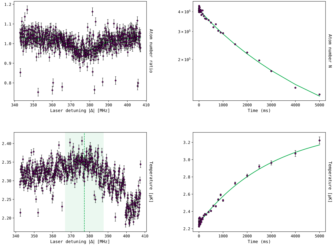
Figure 3.24: Characterization of the molecular line at 375.74 \pm 0.48 MHz in ^{87}\text{Sr} . Panel layout as in Fig. 3.22, with I = 19 \text{ W/cm}^2 for the N(t)/T(t) fits. All detunings are measured from the ^{87}\text{Sr} atomic resonance.
