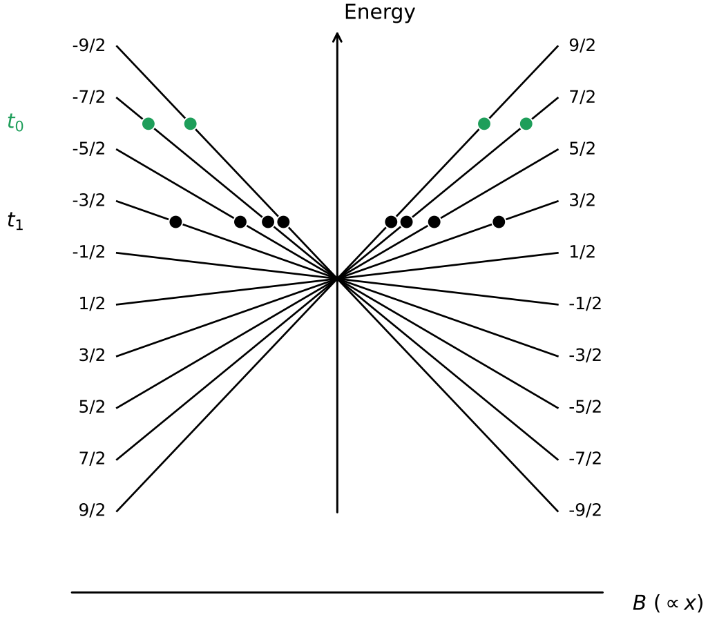
Figure 1.13: Left: spatial dependence of the resonance condition on each m_F sub-level, as a function of position x ( B \propto x ) – adapted from the principle illustrated in Fig. 2.8(d) of [31]. Right: the stirring laser’s frequency, swept in a sawtooth pattern over time in our implementation. At each instant t_0 , the instantaneous frequency (right) is simultaneously resonant with several (m_F, x) pairs (left, black dots); sweeping this frequency over time thus randomizes the m_F population across the whole trap.
