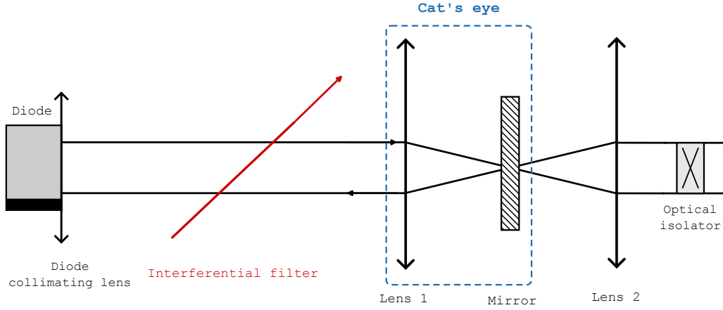
Figure 1.19: External Cavity Diode Laser (ECDL) architecture. A diode lasing at 689 nm is first collimated by a lens, then its frequency is roughly selected by an interference filter marked in red. The beam is focused by a second lens onto a partially reflective mirror (hatched rectangle): together they form a cat’s-eye retroreflector that closes the external cavity, feeding most of the light back for resonant frequency filtering while transmitting a small fraction onward. This output is collimated by a last lens and leaves the laser head through an optical isolator.
