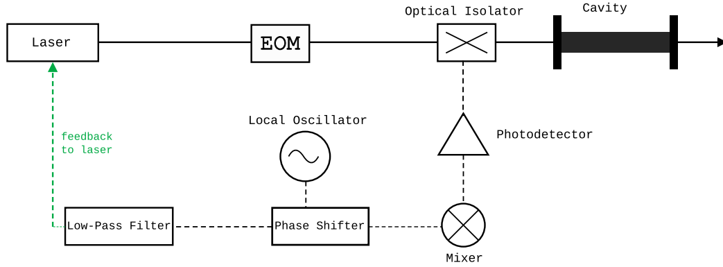
Figure 1.24: Schematic of the Pound-Drever-Hall locking system, extracted and adapted from [5]. The laser is firstly passing through an EOM that is modulating the electric field at frequency f_M , creating two sidebands at frequency f_{\text{laser}} \pm f_M . The carrier at f_{\text{laser}} and the sidebands are passing through the filtering Fabry-Pérot cavity which is reflecting the light going back to the entrance of the cavity. A beamsplitter serving as an optical isolator is reflecting the light to a photodiode. Then this signal is mixed with a local oscillator to extract an error signal to which a low-pass filter is combined to keep only the signal for the locking.
