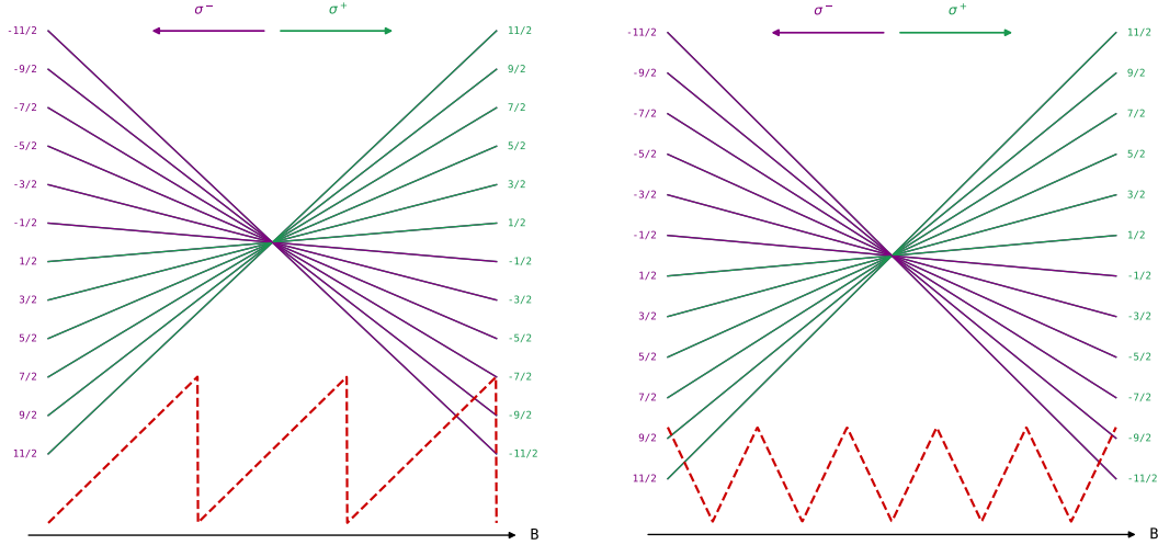
Figure 1.14: Sequential stages of the 689 nm red MOT. From left to right : swap cooling and broadband capture (adapted from [? ]). The size of the cloud is decreasing with the cooling since the atoms are kicked in the opposite direction of the resonant laser of right polarization.
