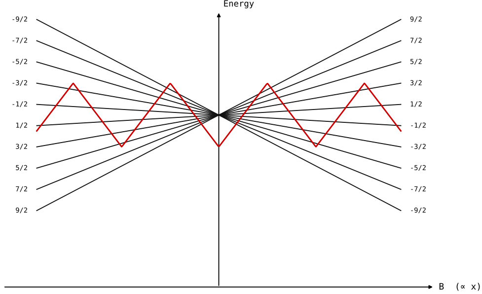
Figure 1.13: Illustration of the melange concept added to the red MOT cooling to capture extreme spin states components inaccessible from the counterpropagating lasers of the red MOT.
