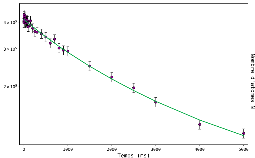
(c) Exponential decay (one- and two-body losses) at the 375.74 MHz resonance.
