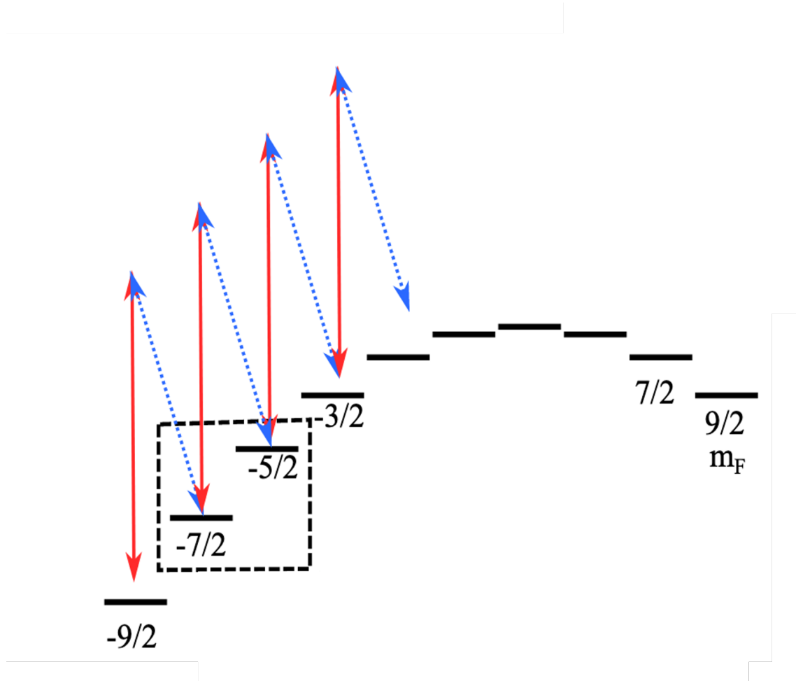
Figure 1.20: Spin manipulation scheme of [4]. The isolation of spin states is allowed by the tensorial shift of the ground states that makes neighbours m_F states isolated from the other resonances.
