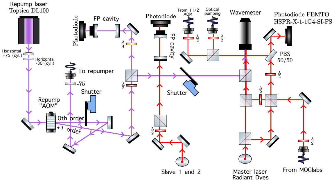
Figure 1.5: Summary of the repumping
