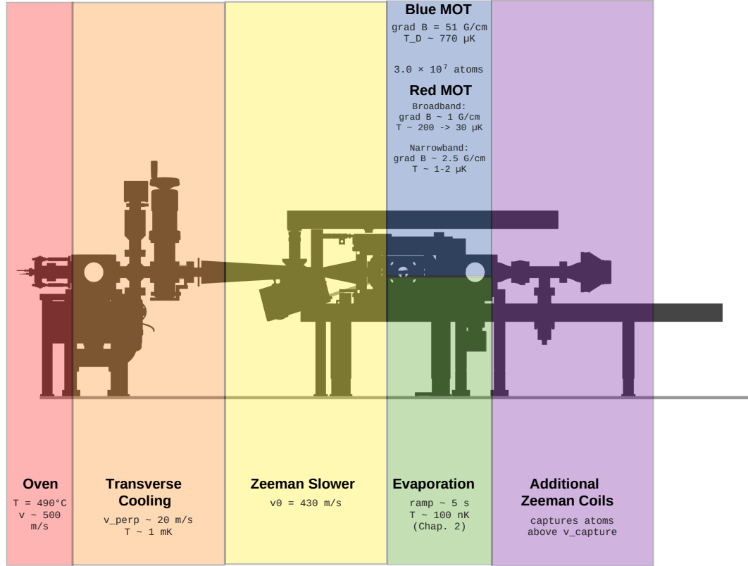
Figure 1.2: Extracted and modified from [1] Experimental full setup for the cooling and trapping of the atoms with figures on the velocity, temperature and typical magnetic gradient on each stage.
