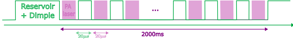
Figure 3.26: Experimental sequence of IR and PA laser chopping to cancel possible coupling to higher energy levels around \lambda = 1064nm that would destruct or decrease collision process. The RF signal of ODT and Raman AOMs is modulated by a GBF at frequency 25 kHz in opposite phases so the atoms in the trap are not lost during the 100\mu s falling time when photoassociated.
