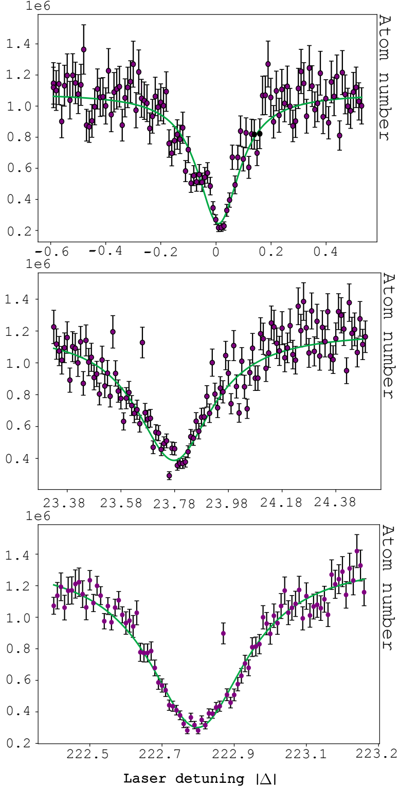
Figure 3.13: ^{88}\text{Sr} atom number (in units of 10^6 atoms) across the intercombination line. (Top) Atomic resonance used as the PA frequency reference. Data points are extracted from 2D Gaussian fits of absorption images; error bars include fit covariance and unperturbed cloud RMS fluctuations. (Middle) \nu = -1 vibrational state ( I = 826 \text{ mW/cm}^2 , 1000 ms). (Bottom) \nu = -2 vibrational state ( I = 303 \text{ mW/cm}^2 , 50 ms). Solid lines are Lorentzian fits with errors accounting for diagonal terms of covariance matrix and systematic fluctuations.
