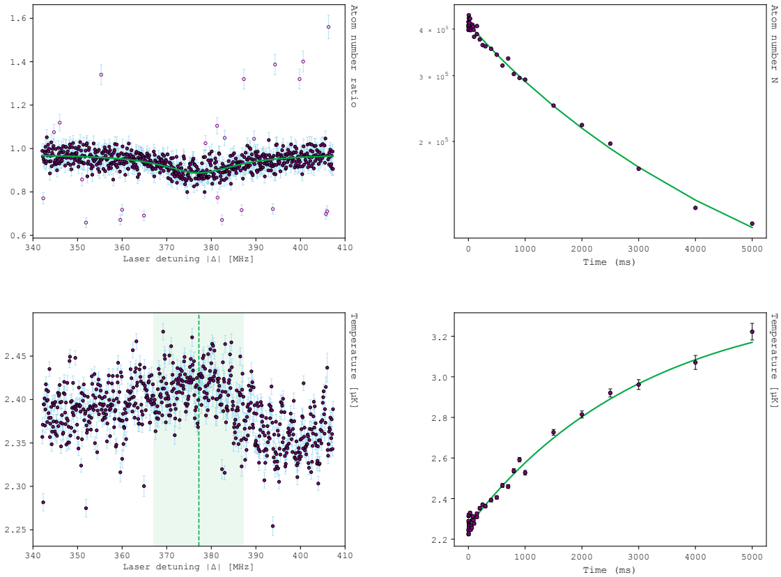
Figure 3.23: Characterization of the molecular line at 377.2 \pm 0.5 MHz in ^{87}\text{Sr} . Panel layout as in Fig. 3.21, with I = 5.6 W/cm 2 for the spectrum and I = 19 W/cm 2 for the N(t)/T(t) fits. Left panels: ratio of the atom numbers of consecutive shots with and without PA light, and temperature of the PA shots computed from the vertical cloud size after time of flight. The Lorentzian fit (green) excludes the points lying more than 3\sigma away from it (open symbols, 24 of 651 points), \sigma = 0.033 being the scatter of the fit residuals. Error bars: 2D Gaussian fit uncertainty, combined in quadrature for the atom number ratio with its relative RMS fluctuation (3.4%) over the first 100 off-resonant points of the scan. All detunings are measured from the ^{87}\text{Sr} atomic resonance.
