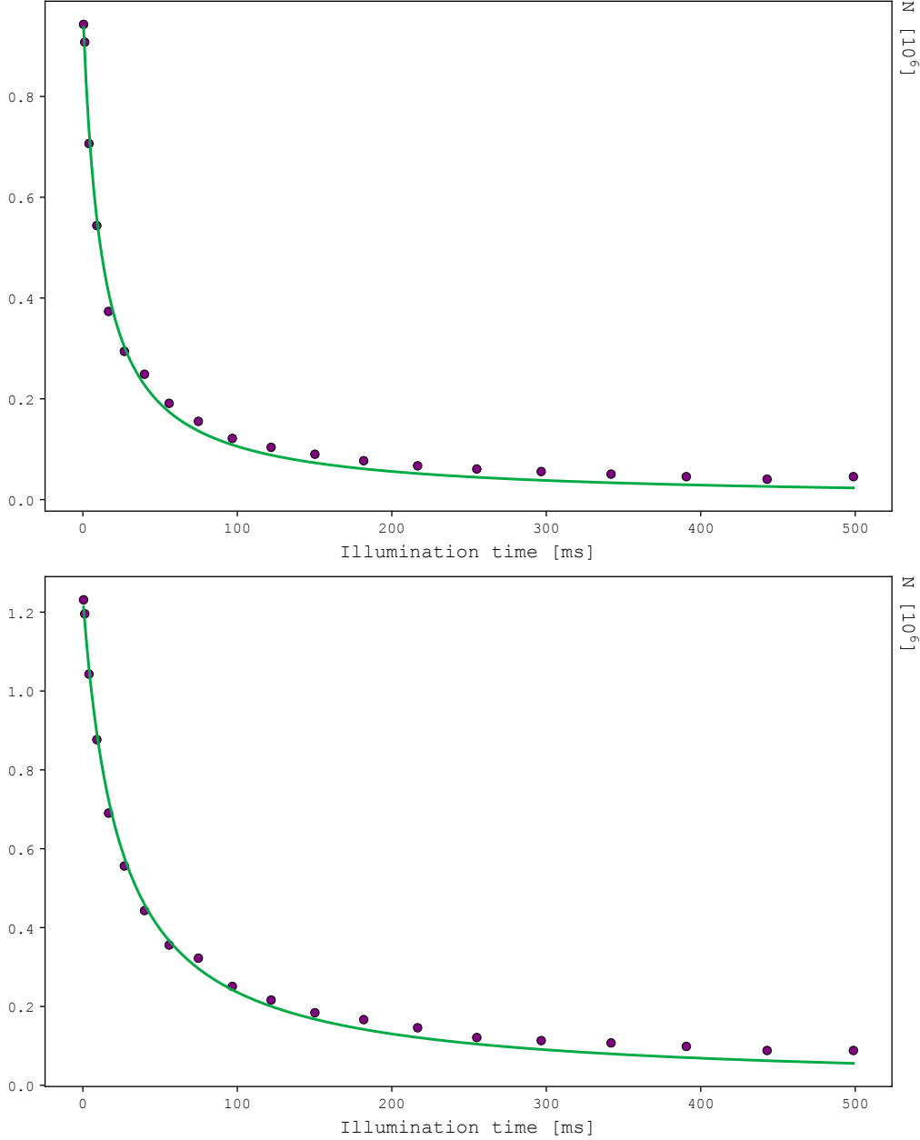
Figure 3.17: Top : atom number decay of ^{88}\text{Sr} of the resonance at f = -23.932(33) MHz. Bottom: atom decay of resonance at f = -222.79(1) MHz. Error bars are not shown, as the original raw data could not be recovered.
