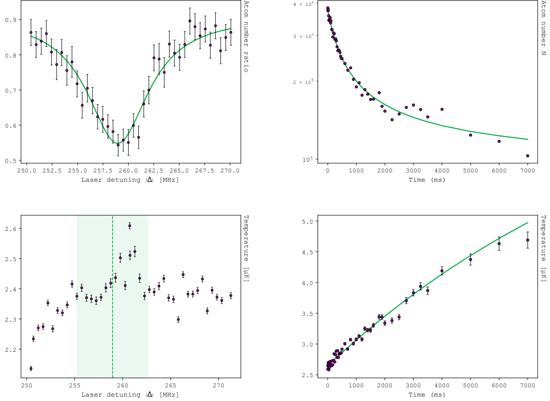
Figure 3.21: Characterization of the molecular line at 259.01 \pm 0.12 MHz in ^{87}\text{Sr} . Top left: resonance spectrum ( I = 19 \text{ W}/\text{cm}^2 , t = 1000 ms), with Lorentzian fit (green). Top right: atom number decay N(t) , fitted via Eq. 3.82 with interpolated T(t) . Bottom left: temperature of the cloud versus detuning; the shaded region and dashed line mark the resonance width and center from the top-left fit. Bottom right: temperature versus illumination time, with a saturating-exponential fit ( \Gamma fixed to the N(t) value). All detunings are measured from the ^{87}\text{Sr} atomic resonance.
