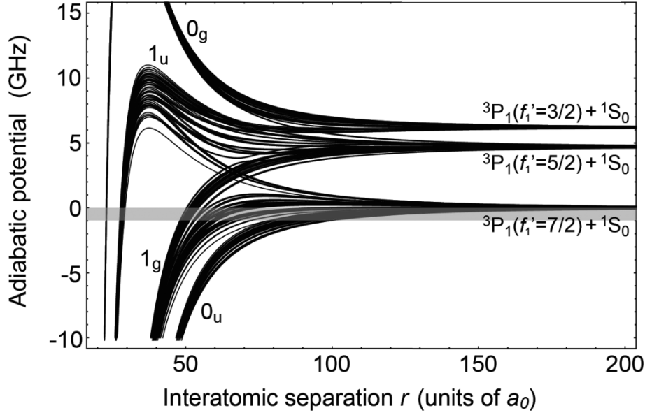
Figure 3.5: Density of molecular potentials for ^{173}\text{Yb} with three hyperfine states, giving rise to numerous triplets of quantum numbers ( T, F, R ). The spectral lines are identified as S_{u/g} , where S is the total orbital momentum projection of the molecule and u/g denotes the electronic parity (see Fig. 3.3).
