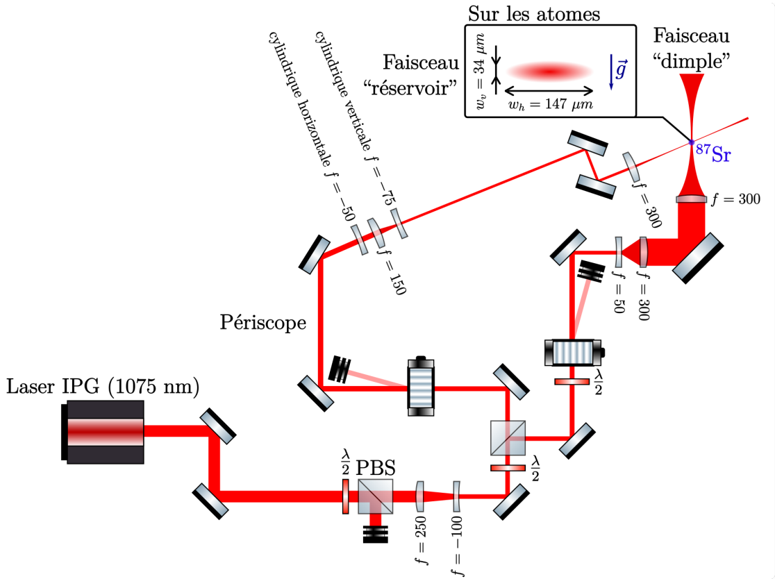
Figure 1.17: Optical layout of the 1075 nm crossed dipole trap laser system.
