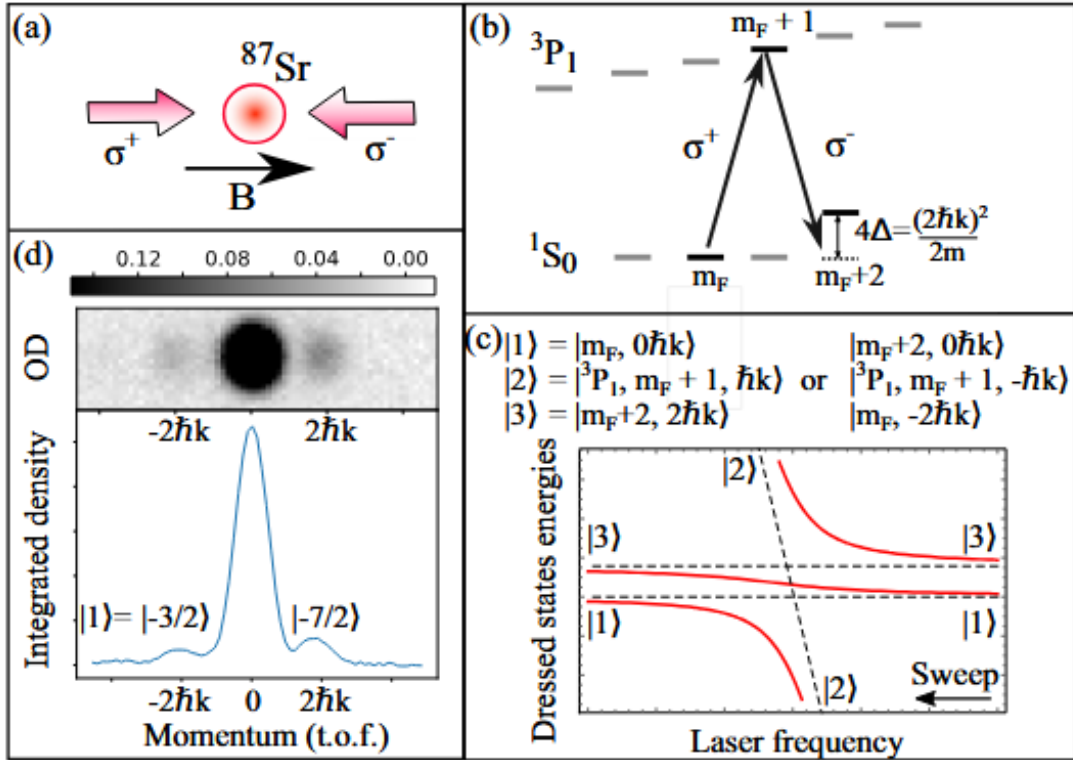
Figure 1.29: Principle of spin-selective detection via coherent momentum transfer ("spin kick"). (a) Counter-propagating beam geometry. (b) Level scheme. (c) Avoided crossing structure for adiabatic transfer. (d) Resulting TOF absorption image showing spatially separated spin components.
