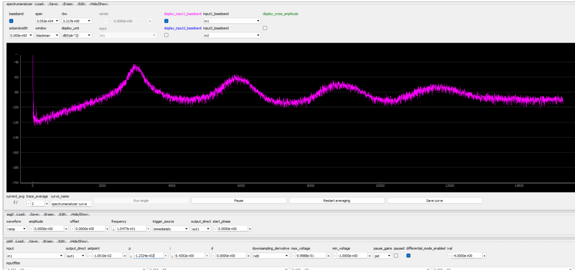
Figure 1.28: Closed-loop noise analysis and mechanical resonance identification using the Red Pitaya.
