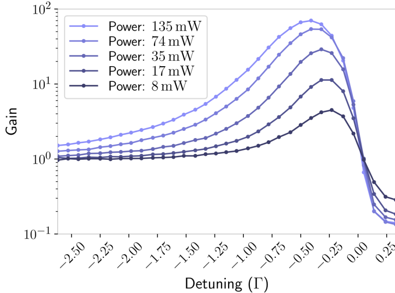
Figure 1.7: Transverse cooling performance as a function of laser detuning and power (adapted from [1]).
