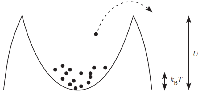
Figure 1.16: Evaporative cooling mechanism in an inclined crossed optical dipole trap, illustrating the escape of high-energy atoms and subsequent re-thermalization.
