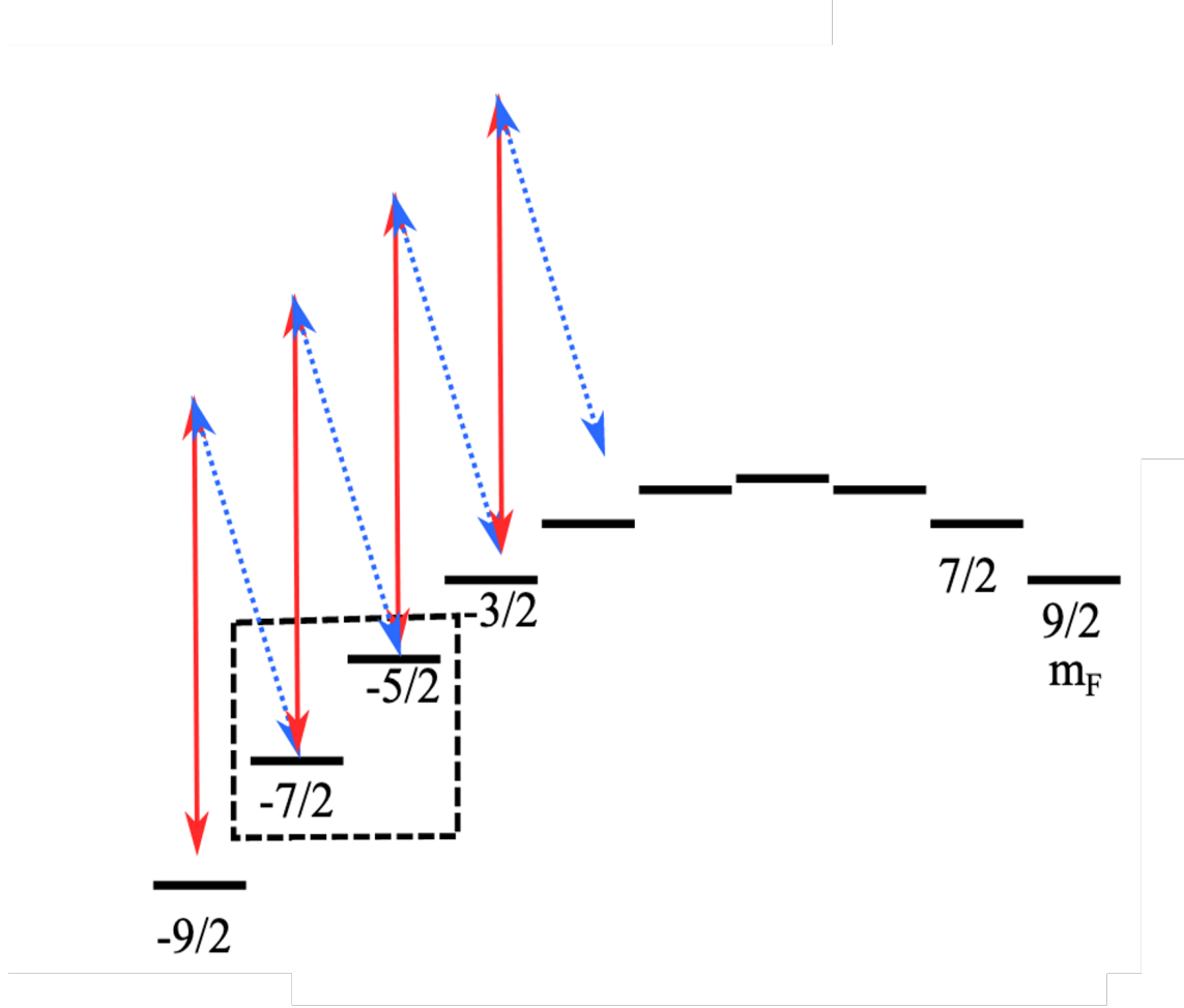
Figure 1.20: Energy level diagram illustrating the Tensorial Light Shift (TLS) and state-selective two-photon Raman transitions.
