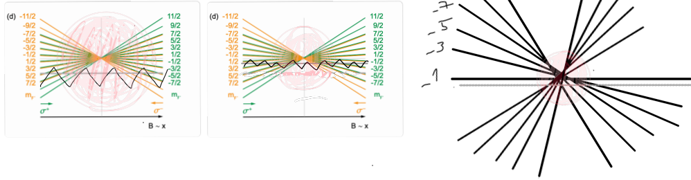
Figure 1.14: Sequential stages of the 689 nm red MOT: broadband capture, compression, and single-frequency cooling (adapted from [? ]).
