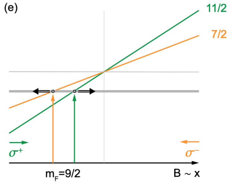
Figure 1.12: Mechanism of population trapping in extreme Zeeman sub-states during the red MOT.
