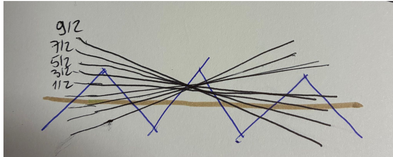
Figure 1.13: Randomization of m_F populations induced by the 689 nm stirring laser.
