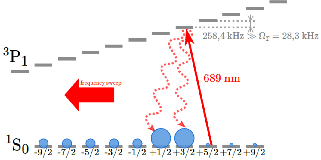
Figure 1.18: Optical pumping scheme on the ^1S_0(F = 9/2) \rightarrow ^3P_1(F = 11/2) transition used to prepare a specific nuclear spin mixture.
