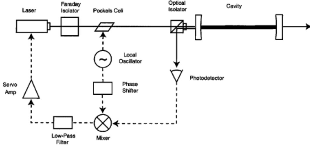
Figure 1.25: Schematic of the PDH locking system, extracted from [3].
