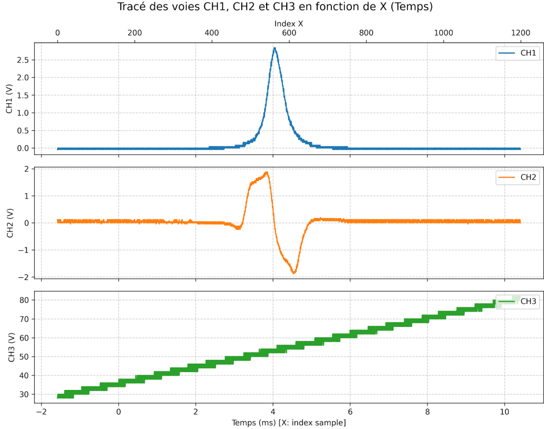
Figure 1.26: Typical Pound-Drever-Hall (PDH) error signal obtained by scanning the cavity length across resonance.
