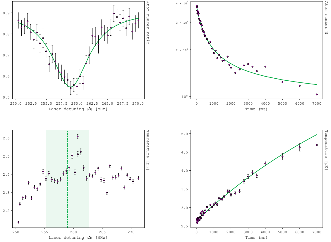
Figure 3.21: Characterization of the molecular line at 259.01 \pm 0.12 MHz in ^{87}\text{Sr} . Top left: resonance spectrum ( I = 19 \pm 1.1 W/cm ^2 , t = 1000 ms, \langle n \rangle = (7.0 \pm 1.0) \times 10^{12} cm ^{-3} ), with Lorentzian fit (green). Top right: atom number decay N(t) (same intensity and density), fitted via Eq. 3.82 with interpolated T(t) . Bottom left: temperature of the cloud versus detuning; the shaded region and dashed line mark the resonance width and center from the top-left fit. Bottom right: temperature versus illumination time, with a saturating-exponential fit ( \Gamma fixed to the N(t) value). All detunings are measured from the ^{87}\text{Sr} atomic resonance.
