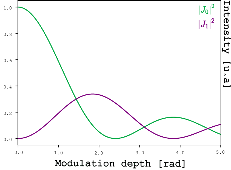
Figure 3.10: Modulus square of the 0^{\text{th}} and 1^{\text{st}} Bessel functions J_n governing the power distribution between the carrier and PDH sidebands.
