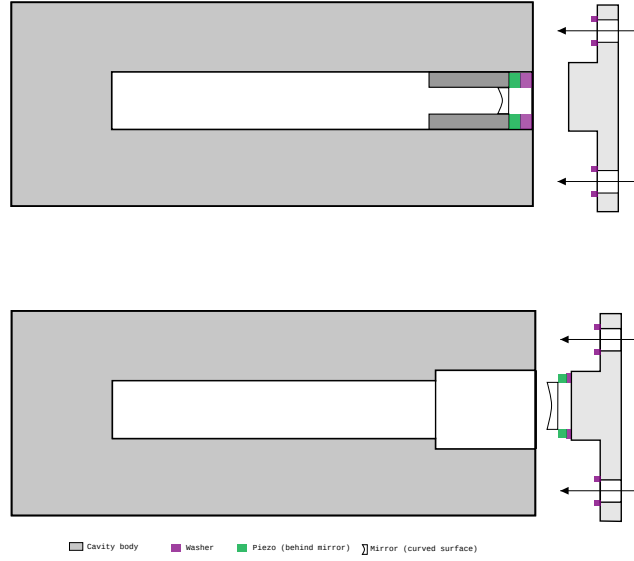
Figure 1.22: Top : Initial fixed cavity assembly using glued mirrors, lacking mechanical alignment degrees of freedom. Bottom : Upgraded and final cavity mount featuring three adjustment screws and compliant washers for precise angular and longitudinal alignment
