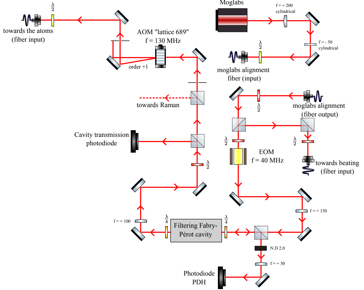
Figure 1.21: Complete optical setup including the Fabry-Pérot cavity and PDH stabilization loop.
