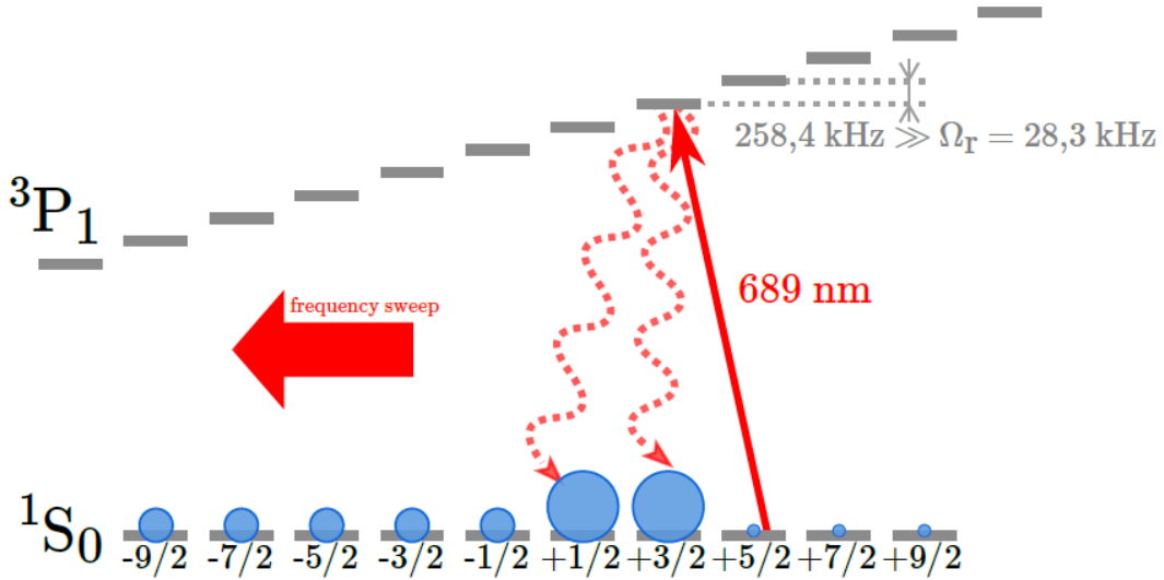
Figure 1.17: Optical pumping scheme on the ^1S_0(F = 9/2) \rightarrow ^3P_1(F = 11/2) transition used to prepare a specific nuclear spin mixture. The red laser is ramped through the target energy level of ^3P_1 : the atoms decay to neighbours states m_F \pm 1 of ^1S_0
