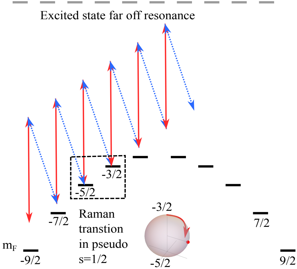
Figure 1.19: Spin manipulation scheme of [1]. The isolation of spin states is allowed by the tensorial shift of the ground states that makes neighbours m_F states isolated from the other resonances.
