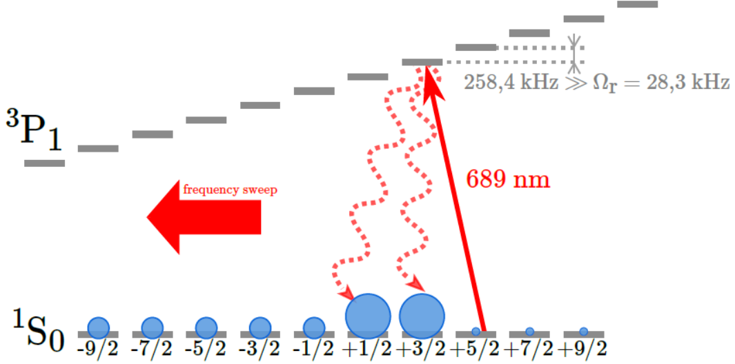
Figure 1.12: Optical pumping scheme on the ^1S_0(F = 9/2) \rightarrow ^3P_1(F = 11/2) transition used to prepare a specific nuclear spin mixture.
