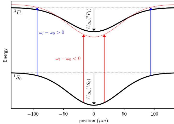
Figure 1.9: Principle of localized 689 nm MOT loading inside the crossed optical dipole trap due to the differential AC Stark shift between ^1S_0 and ^3P_1 .
