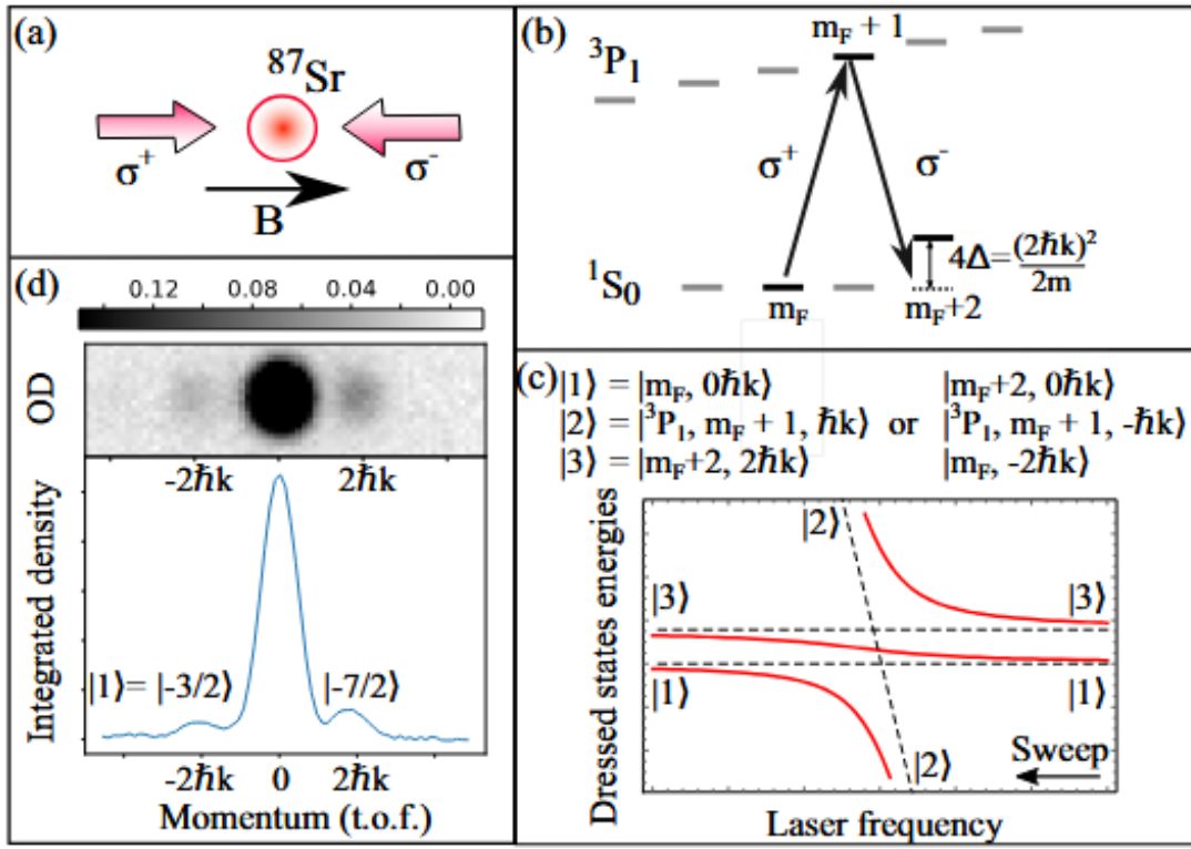
Figure 1.18: Principle of spin-selective detection via coherent momentum transfer ("spin kick"). (a) Counter-propagating beam geometry. (b) Level scheme. (c) Avoided crossing structure for adiabatic transfer. (d) Resulting TOF absorption image showing spatially separated spin components.
