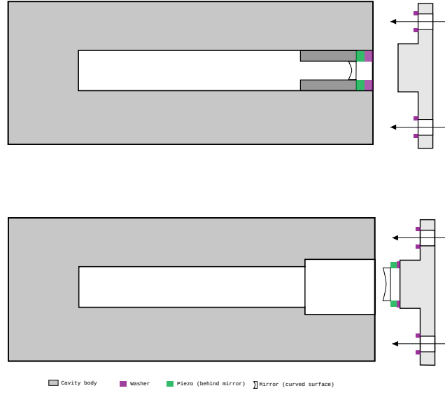
Figure 1.23: Top : Initial fixed cavity assembly using glued mirrors, lacking mechanical alignment degrees of freedom. Bottom : Upgraded and final cavity mount featuring three adjustment screws and compliant washers for precise angular and longitudinal alignment
