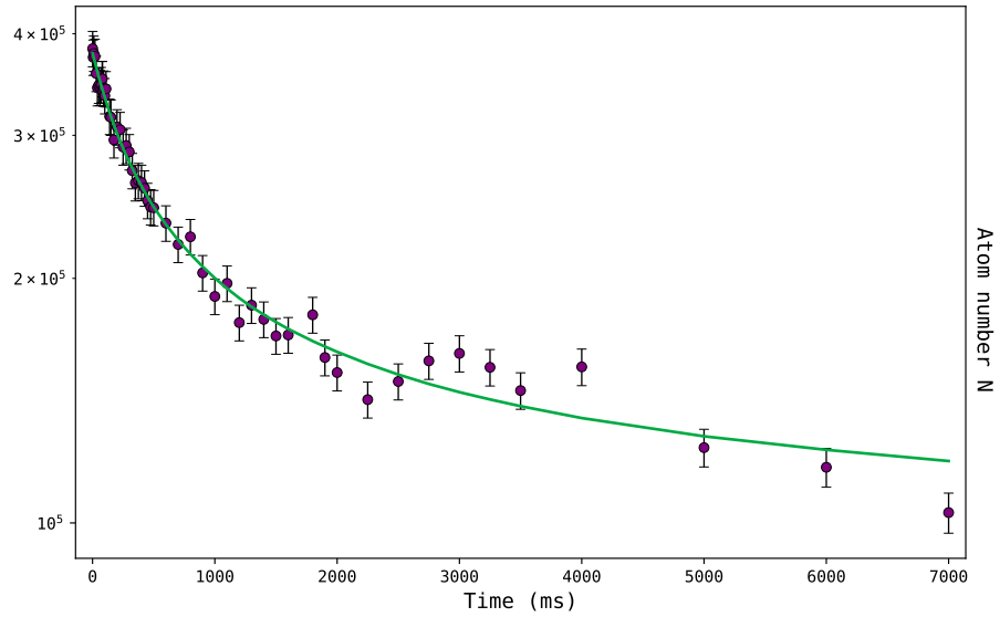
(c) dN/dt measurement at the 259.01 MHz resonance.
