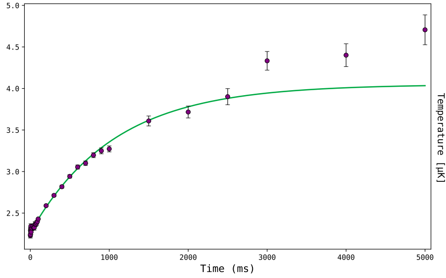
(b) Temperature of the gas at the 276.83 MHz resonance.
