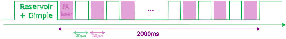
Figure 3.25: Experimental sequence of the ODT and PA laser chopping used to prevent multi-photon transitions to higher energy levels. The RF signals driving the ODT and Raman AOMs are modulated at 25 kHz in opposite phase. This ensures that the two lasers do not overlap while keeping the extinction time short enough to avoid atom loss due to gravity.
