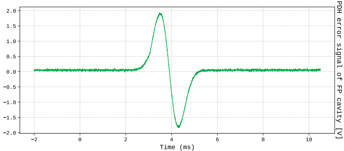
Figure 1.26: Typical Pound-Drever-Hall (PDH) error signal obtained by scanning the cavity length across resonance.
