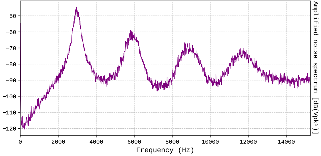
Figure 1.28: Closed-loop noise analysis and mechanical resonance identification using the Red Pitaya.
