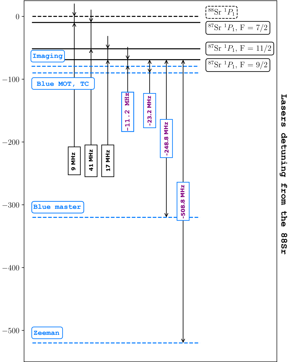
Figure 1.5: Diagram of the frequencies of each laser composing the blue chain of the blue MOT broadband cooling. Blue dashed lines indicate the tunable frequencies of the lasers. Plain black lines indicate the transitions of ^{87}\text{Sr} and ^{88}\text{Sr} isotopes.
