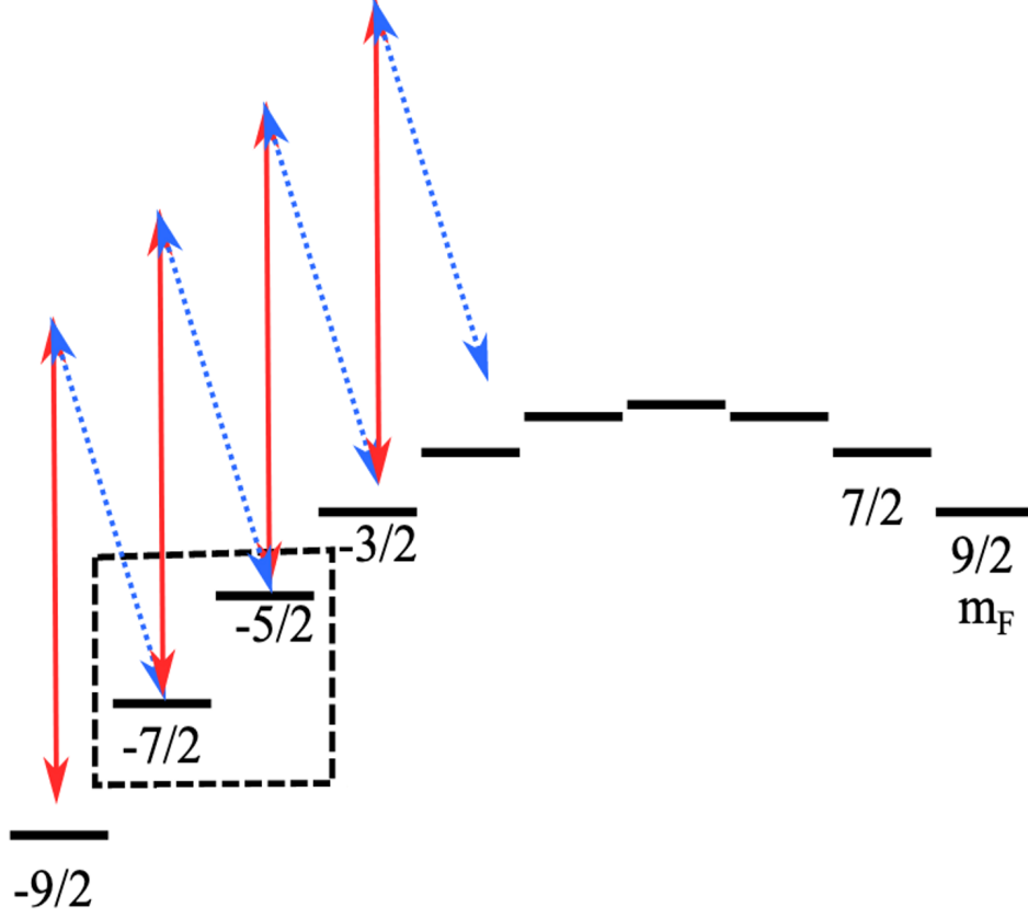
Figure 1.20: Energy level diagram illustrating the Tensorial Light Shift (TLS) and state-selective two-photon Raman transitions.
