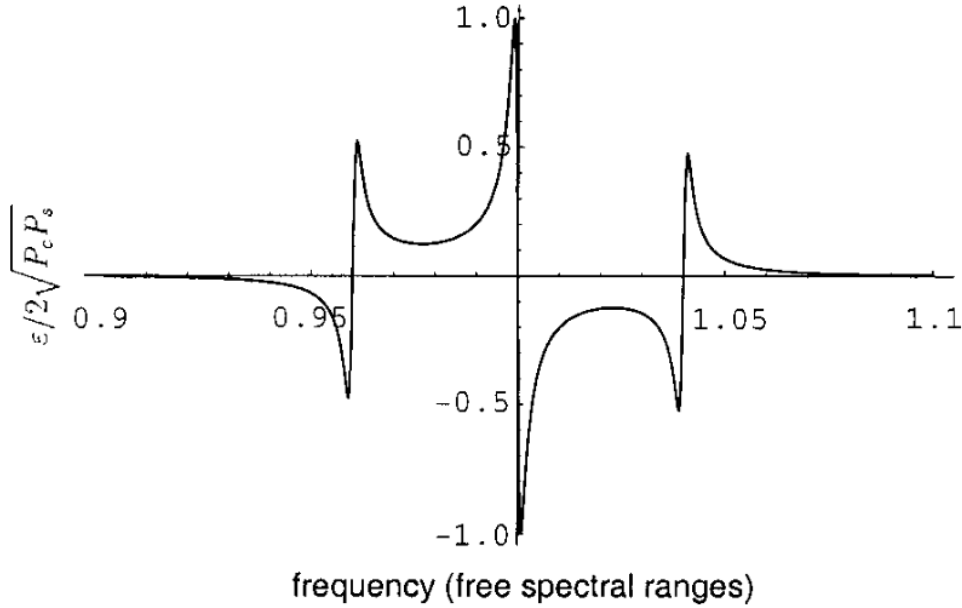
Figure 1.19: Typical Pound-Drever-Hall (PDH) error signal obtained by scanning the cavity length across resonance.
