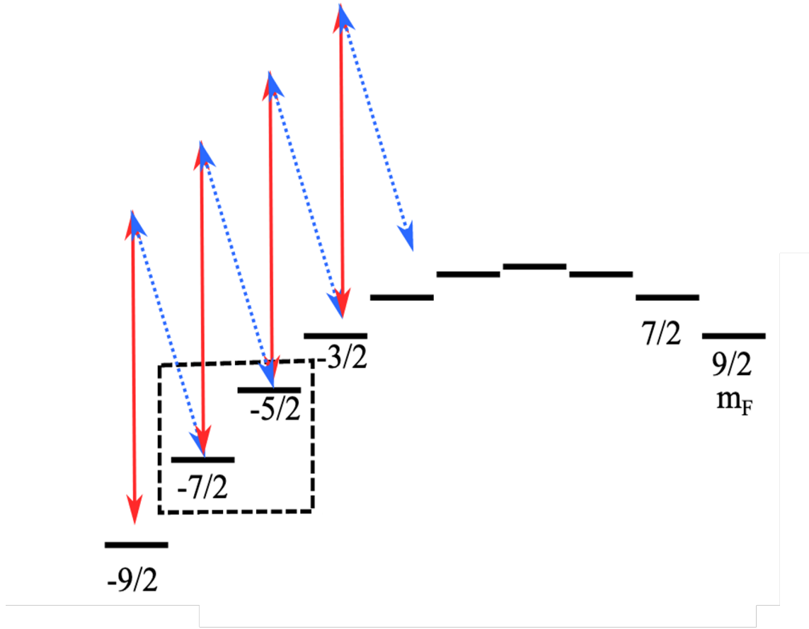
Figure 1.16: Energy level diagram illustrating the Tensorial Light Shift (TLS) and state-selective two-photon Raman transitions.
