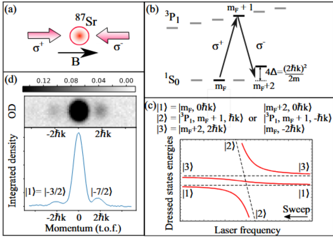
Figure 1.20: Principle of spin-selective detection via coherent momentum transfer ("spin kick"). (a) Counter-propagating beam geometry. (b) Level scheme. (c) Avoided crossing structure for adiabatic transfer. (d) Resulting TOF absorption image showing spatially separated spin components.
