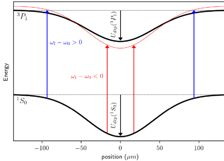
Figure 1.11: Principle of localized 689 nm MOT loading inside the crossed optical dipole trap due to the differential AC Stark shift between ^1S_0 and ^3P_1 .
