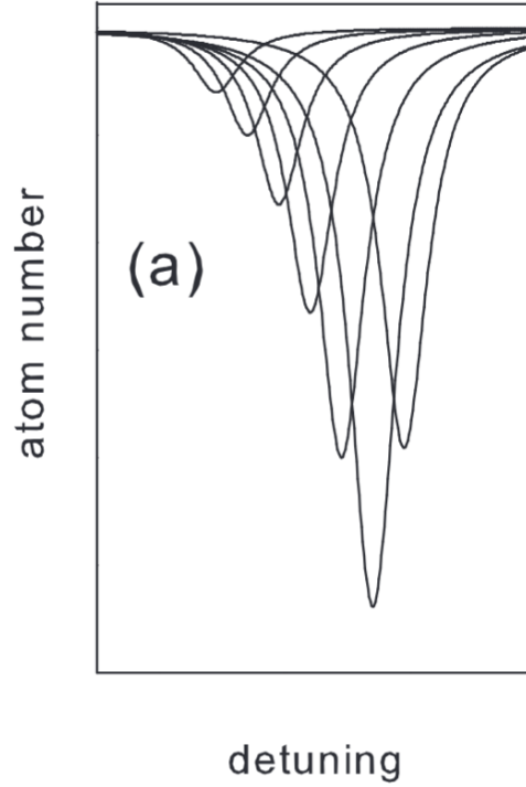
Figure 1.3: Illustration of the Doppler cooling effect: velocity classes are shifted relative to the atomic resonance frequency \omega_0 .
