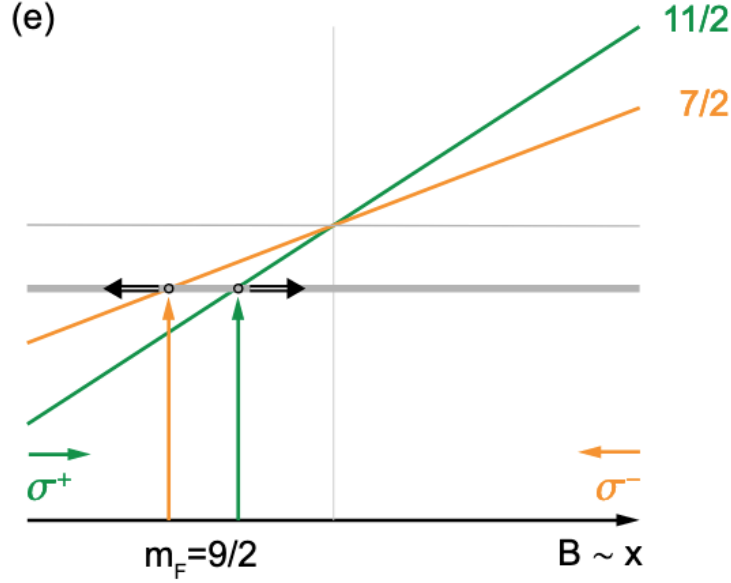
Figure 1.8: Mechanism of population trapping in extreme Zeeman sub-states during the red MOT.
