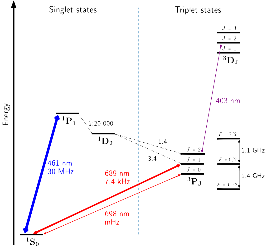
Figure 1.1: Extracted from [2] Energy spectrum of ^{87}\text{Sr} including fine and hyperfine interactions. In blue the 461 nm transition used for TC, Zeeman cooling, blue MOT stage and imaging. The purple arrow indicates the repump line at 403 nm from the metastable state ^3P_2 used for the atoms leaking from the intermediate ^1D_2 state. In red the transition to ^3P_1 at 689 nm used for all stages of the red MOT, optical pumping, spin manipulation, coherent manipulation (see Chap.2), photoassociation (see Chap.3, through the different hyperfine states F = 7/2, 9/2, 11/2 ). The 698 nm transition indicates the clock transition which we do not use in this experiment.
