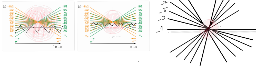
Figure 1.13: Sequential stages of the 689 nm red MOT: broadband capture, compression, and single-frequency cooling (adapted from [? ]).
