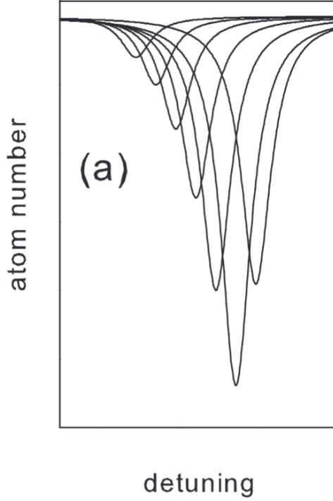
Figure 1.5: Illustration of Doppler cooling: velocity classes are shifted relative to the atomic resonance frequency \omega_0 .
