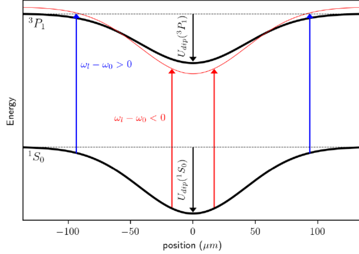
Figure 1.14: Simulation extracted from [2]. Principle of localized 689 nm MOT loading inside the crossed optical dipole trap due to the differential AC Stark shift between ^1S_0 and ^3P_1 .
