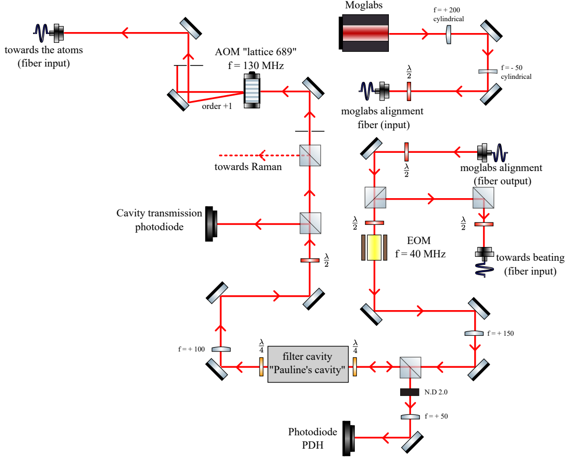
Figure 1.21: Complete optical setup including the Fabry-Pérot cavity and PDH stabilization loop.
