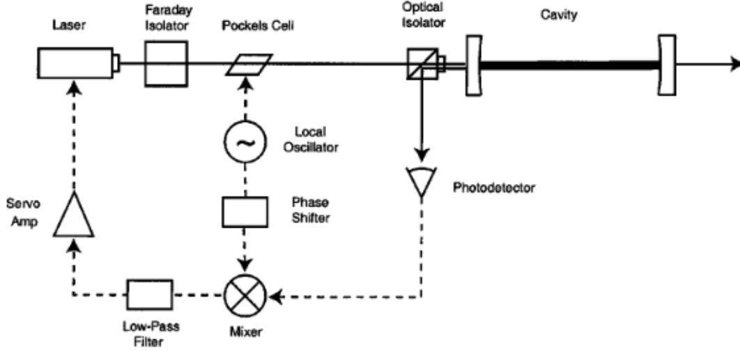
Figure 1.24: Schematic of the PDH locking system, extracted from [3].
