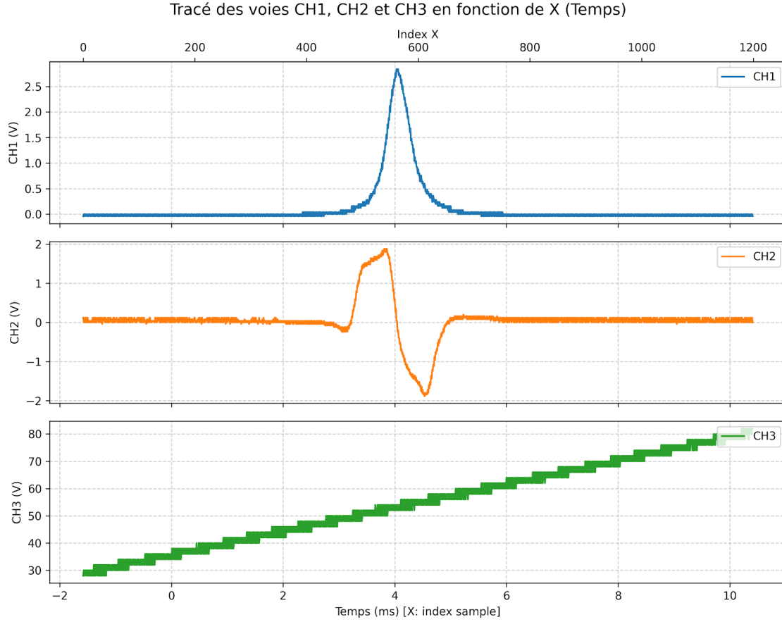
Figure 1.25: Typical Pound-Drever-Hall (PDH) error signal obtained by scanning the cavity length across resonance.
