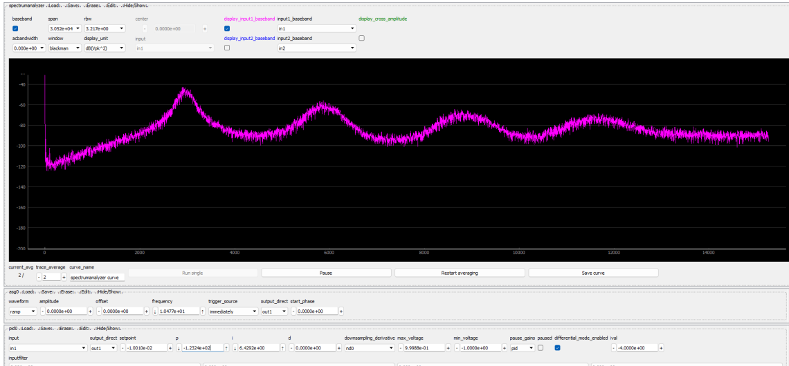
Figure 1.27: Closed-loop noise analysis and mechanical resonance identification using the Red Pitaya.
