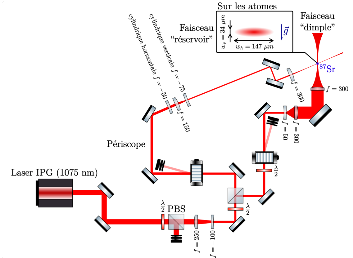
Figure 1.16: Optical layout of the 1075 nm crossed dipole trap laser system.
