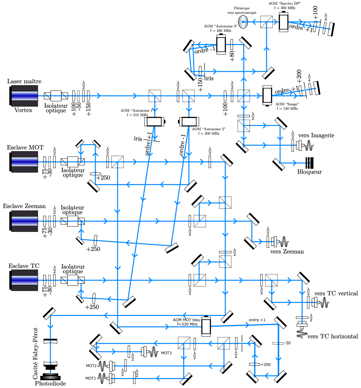
Figure 1.3: Optical layout of the 461 nm blue laser system for transverse cooling, Zeeman slowing, and blue MOT.
