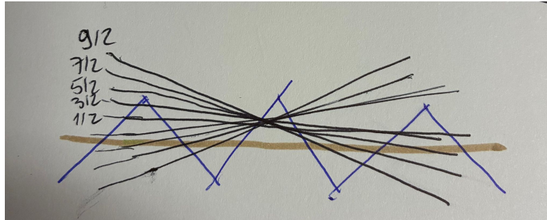
Figure 1.12: Randomization of m_F populations induced by the 689 nm stirring laser.
