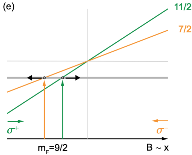
Figure 1.11: Mechanism of population trapping in extreme Zeeman sub-states during the red MOT.
