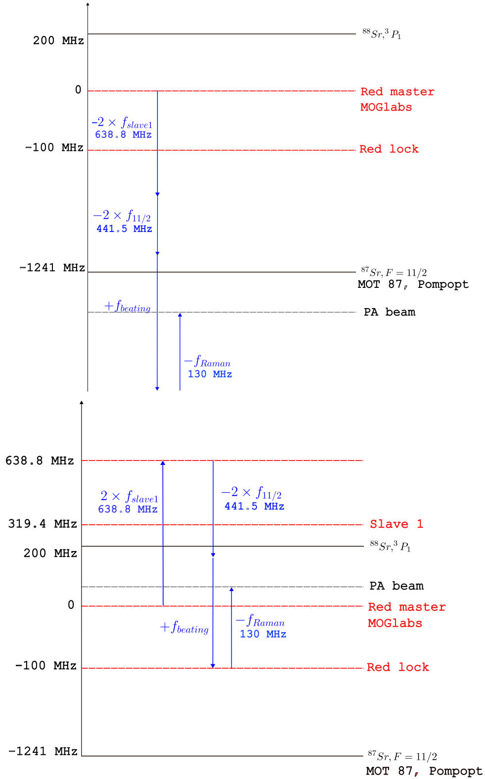
Figure 3.9: Frequency schemes for photoassociation (PA) depending on the targeted isotope: (top) scheme for ^{87}\text{Sr} and (bottom) scheme for ^{88}\text{Sr} . Switching the diffracted order of 'AOM Slave 1' allows for a seamless transition between isotopes, requiring only a minor realignment of the beam injection downstream of the AOM.
