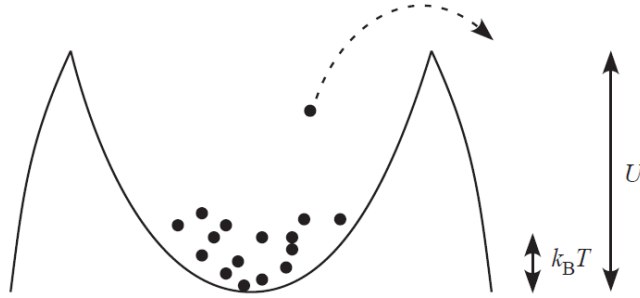
Figure 1.15: Evaporative cooling mechanism in an inclined crossed optical dipole trap, illustrating the escape of high-energy atoms and subsequent re-thermalization.
