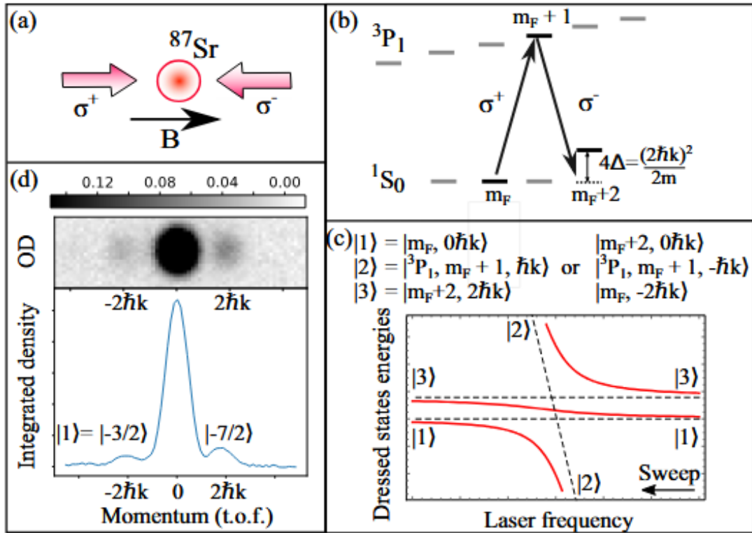
Figure 1.28: Principle of spin-selective detection via coherent momentum transfer ("spin kick"). (a) Counter-propagating beam geometry. (b) Level scheme. (c) Avoided crossing structure for adiabatic transfer. (d) Resulting TOF absorption image showing spatially separated spin components.
