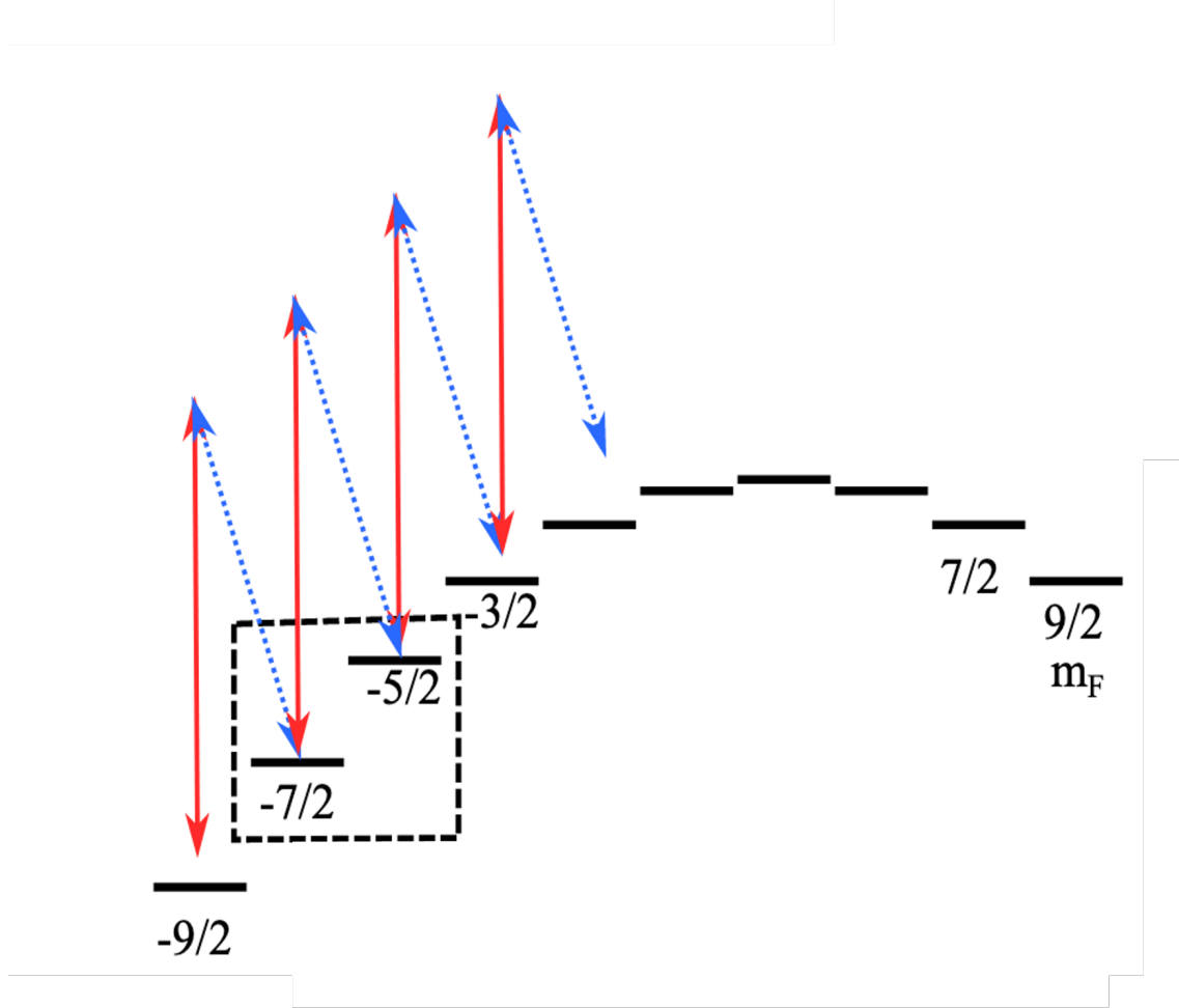
Figure 1.19: Energy level diagram illustrating the Tensorial Light Shift (TLS) and state-selective two-photon Raman transitions.
