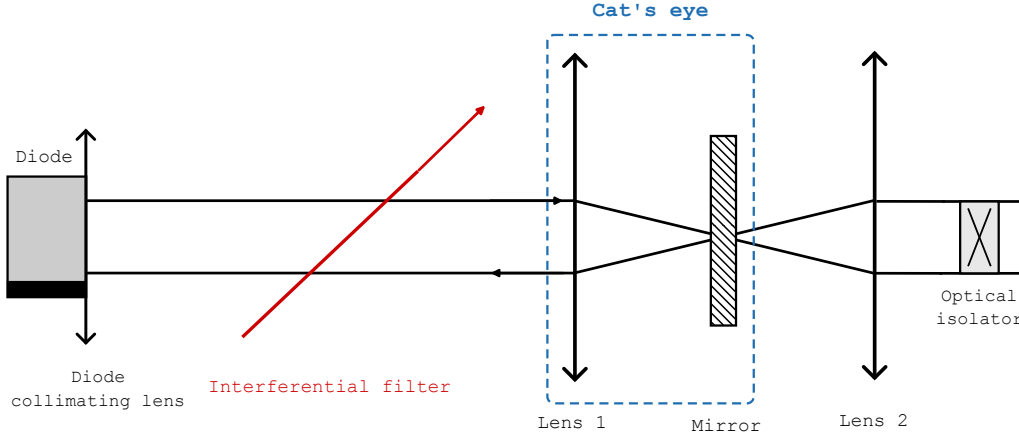
Figure 1.19: MOGlabs External Cavity Diode Laser (ECDL) architecture used for spin manipulation. A diode lasing at 689 nm is first collimated by a lens, then its frequency is roughly selected by an interference filter marked in red. The beam is focused by a second lens onto a partially reflective mirror (hatched rectangle): together they form a cat's-eye retroreflector that closes the external cavity, feeding most of the light back for resonant frequency filtering while transmitting a small fraction onward. This output is collimated by a last lens and leaves the laser head through an optical isolator.
