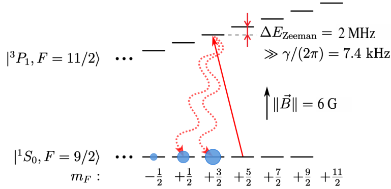
Figure 1.18: Optical pumping scheme on the ^1S_0(F = 9/2) \rightarrow ^3P_1(F = 11/2) transition used to prepare a specific nuclear spin mixture. The red laser is ramped through the target energy level of ^3P_1 : the atoms decay to neighbours states m_F \pm 1 of ^1S_0
