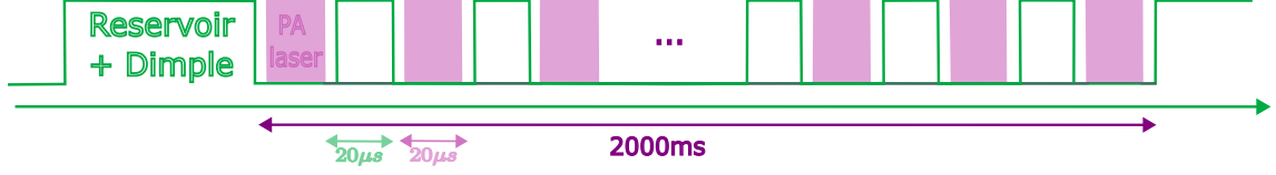
Figure 3.24: Experimental sequence of the ODT and PA laser chopping used to prevent multi-photon transitions to higher energy levels. The RF signals driving the ODT and Raman AOMs are modulated at 25 kHz in opposite phase. This ensures that the two lasers do not overlap while keeping the extinction time short enough to avoid atom loss due to gravity.
