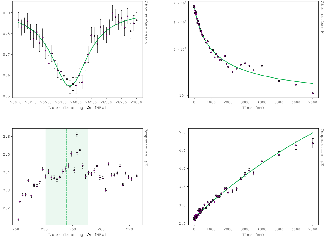
Figure 3.21: Characterization of the molecular line at -259.01 \pm 0.12 MHz in ^{87}\text{Sr} . Top left: resonance spectrum ( I = 19.0 \pm 1.1 W/cm ^2 , t = 1000 ms, \langle n \rangle = (7.0 \pm 1.0) \times 10^{12} cm ^{-3} ), with Lorentzian fit (green). Top right: atom number decay N(t) (same intensity and density), fitted via Eq. 3.77 with interpolated T(t) . Bottom left: temperature of the cloud versus detuning; the shaded region and dashed line mark the resonance width and center from the top-left fit. Bottom right: temperature versus illumination time, fitted with the empirical saturating exponential of Eq. 3.92, with the one-body loss rate \Gamma fixed to the value obtained from the fit of N(t) . All detunings are measured from the ^{87}\text{Sr} atomic resonance.
