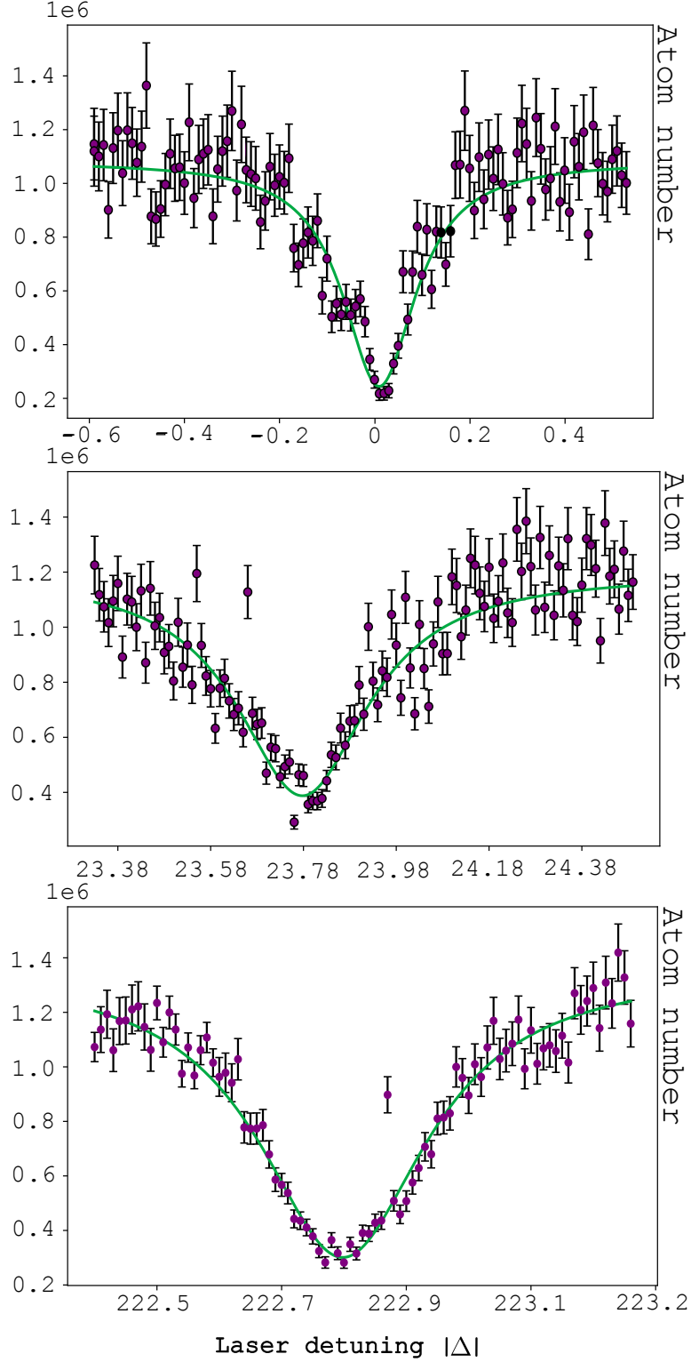
Figure 3.13: ^{88}\text{Sr} atom number (in units of 10^6 atoms) across the intercombination line. (Top) Atomic resonance used as the PA frequency reference ( I = 276 \pm 22 \mu\text{W}/\text{cm}^2 , 80 ms, \bar{\omega}/2\pi = 213 \pm 10 Hz, \langle n \rangle = (4.5 \pm 0.6) \times 10^{13} \text{ cm}^{-3} , T = 1.4 \mu\text{K} ). Data points are extracted from 2D Gaussian fits of absorption images; error bars include fit covariance and unperturbed cloud RMS fluctuations. (Middle) \nu = -1 vibrational state ( I = 7.3 \pm 0.6 \text{ mW}/\text{cm}^2 , 1000 ms, \bar{\omega}/2\pi = 181 \pm 9 Hz, \langle n \rangle = (1.8 \pm 0.3) \times 10^{13} \text{ cm}^{-3} , T = 1.8 \mu\text{K} ). (Bottom) \nu = -2 vibrational state ( I = 826 \pm 66 \text{ mW}/\text{cm}^2 , 10 ms, \bar{\omega}/2\pi = 184 \pm 9 Hz, \langle n \rangle = (3.0 \pm 0.4) \times 10^{13} \text{ cm}^{-3} , T = 1.4 \mu\text{K} ). The intensity uncertainties only include the 4% uncertainty on the waist. Solid lines are Lorentzian fits with errors accounting for diagonal terms of covariance matrix and systematic fluctuations.
