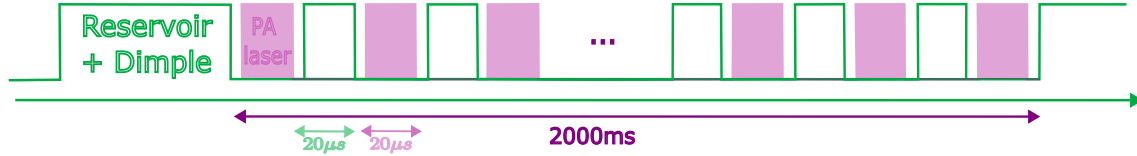
Figure 3.26: Experimental sequence of the ODT and PA laser chopping used to prevent multi-photon transitions to higher energy levels. The RF signals driving the ODT and Raman AOMs are modulated at 25 kHz in opposite phase. This ensures that the two lasers do not overlap while keeping the extinction time short enough to avoid atom loss due to gravity.
